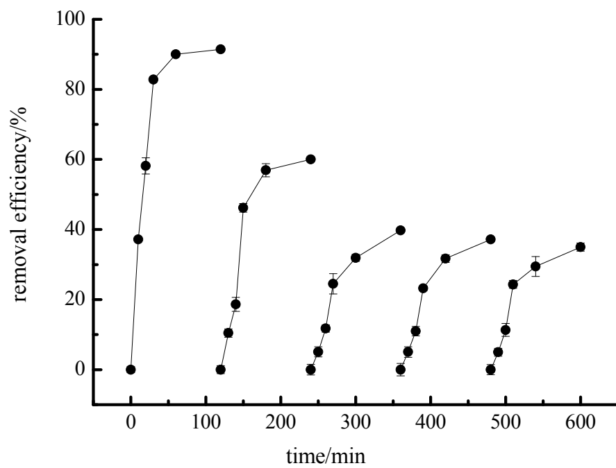
Fig. SM-1 Effect of different reuse times of the Pd/TiO 2 TNs/Ti electrode on 2,4-DCP dechlorination. (Electrolyte: 50 mmol·L -1 Na 2 SO 4 and 20 mg·L -1 2,4-DCP; pH 5.5; cathode potential: -0.7 V)
