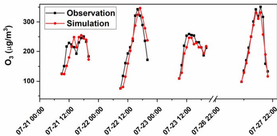
Figure. S1 Day-to-day comparison of observed and simulated O 3 concentration.
