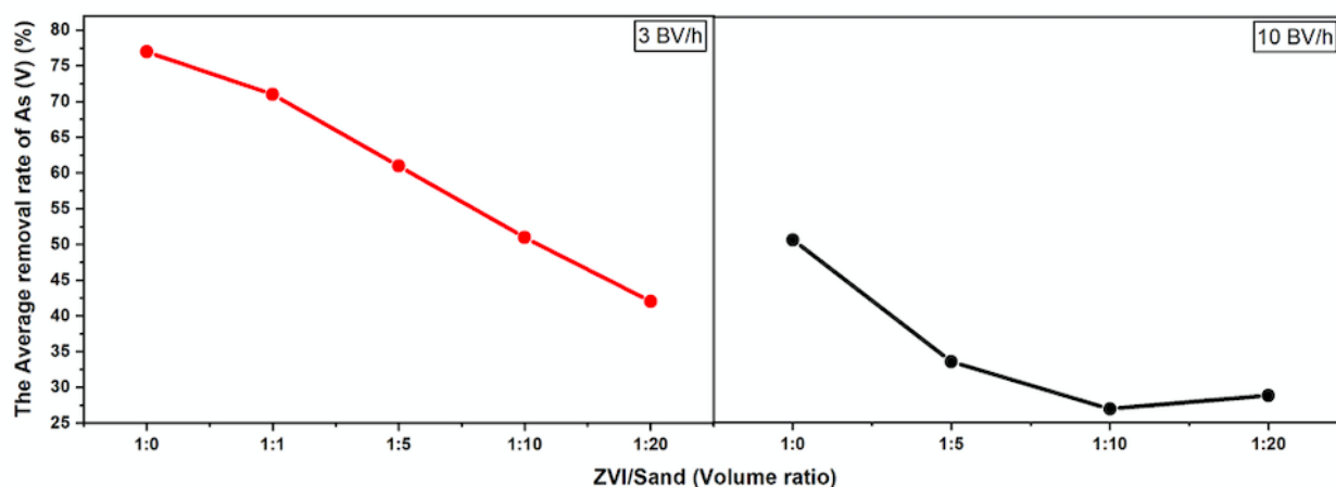
Fig. S1. Average arsenic removal at various ratios of ZVI/sand columns
