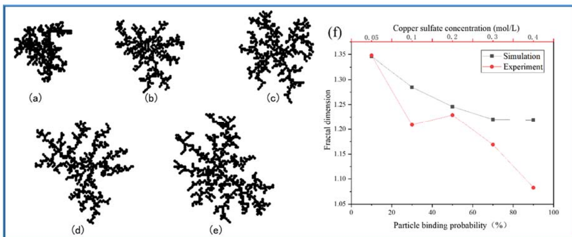
Fig. S3 Morphologies and fractal dimensions of agglomerates with different particle numbers and ion concentration.
