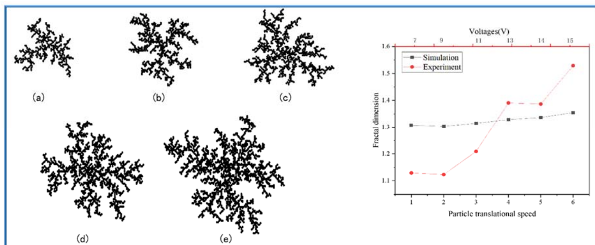
Fig. S2 Morphologies and fractal dimensions of agglomerates with different particle translational speed and voltage.
