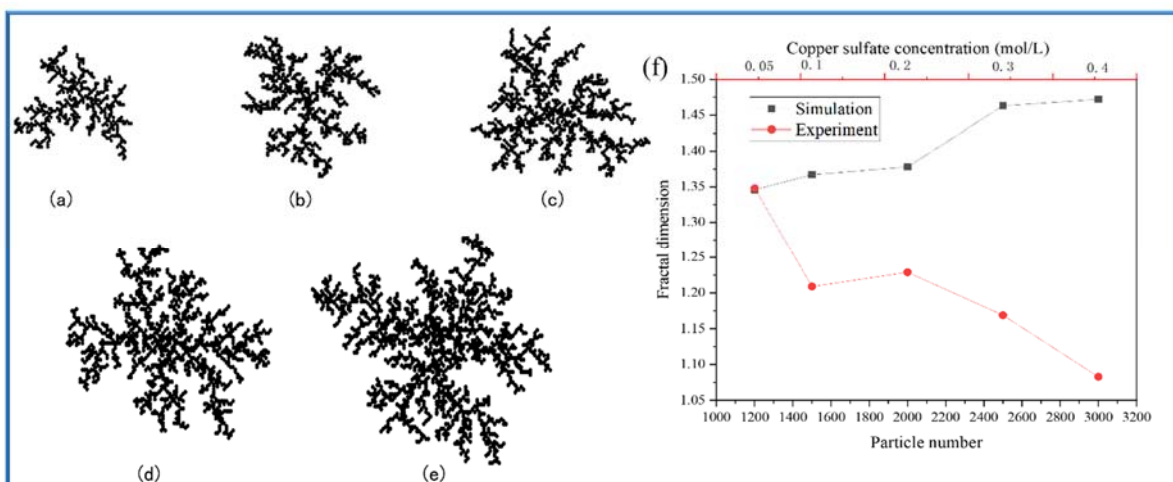
Fig. S4 Morphologies and fractal dimensions of agglomerates with different particle binding probability and ion concentration.
