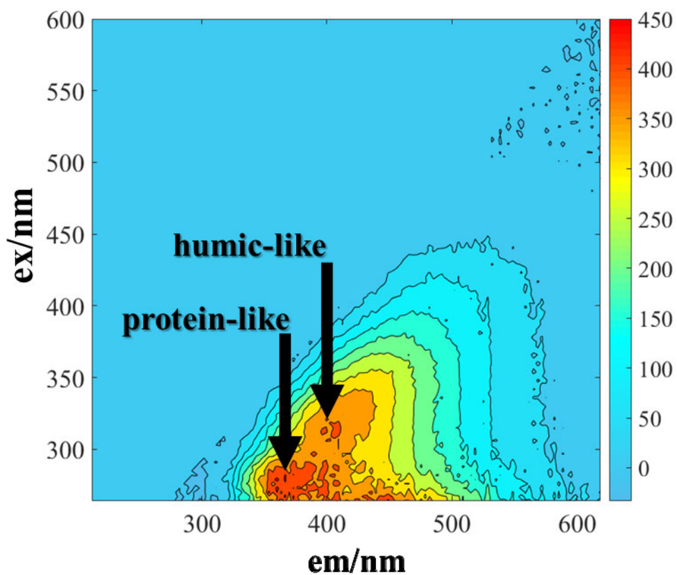
Fig. S2 Typical EEM of the sample from Zhuzhuanjing WWTP
