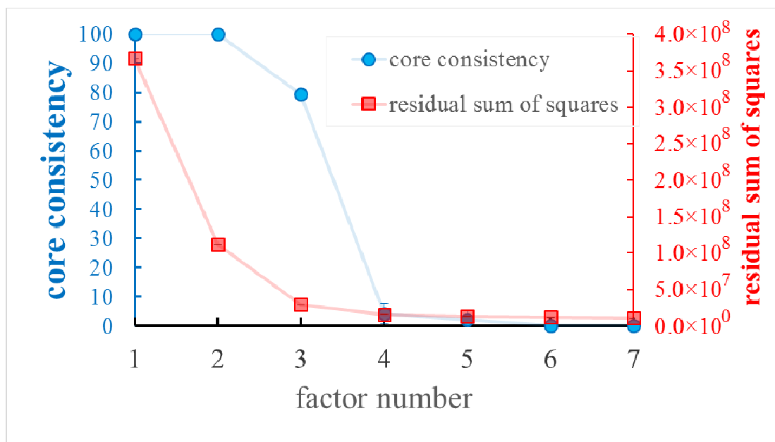
Fig. S3 Core consistency and RSS of different factors using PARAFAC
