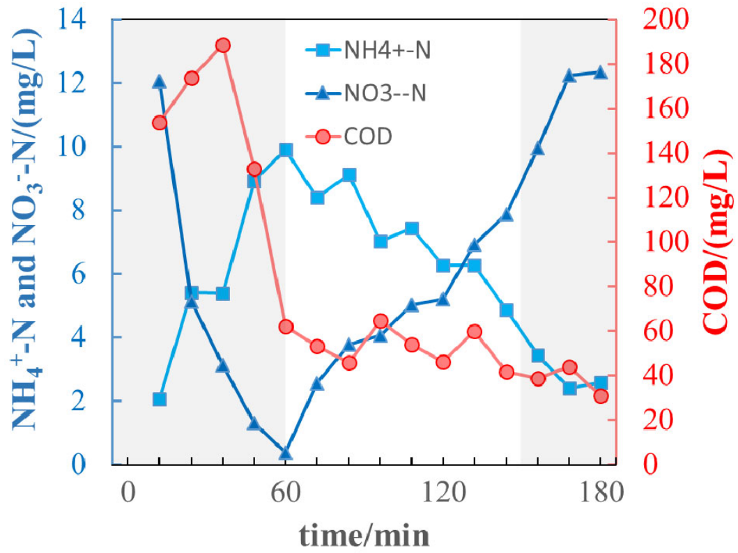
Fig. S1 COD, ammonia and nitrate concentration profiles of Zhuzhuanjing WWTP in an operating cycle
