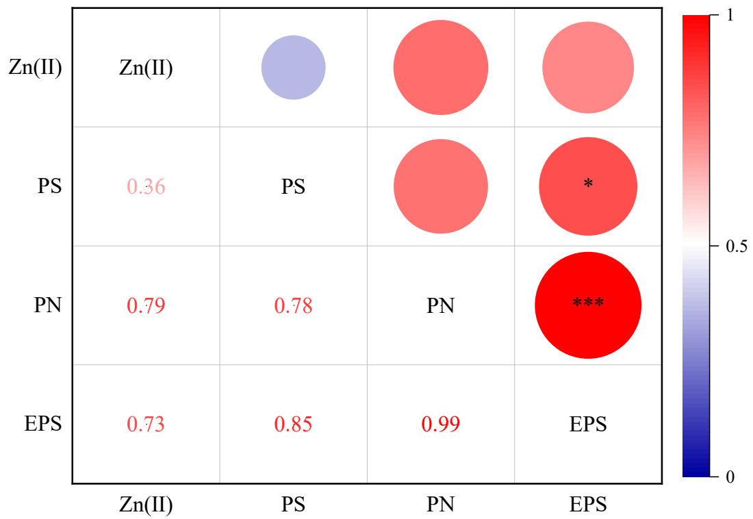
Fig. S1. Pearson correlation analysis between Zn(II) and EPS component.
