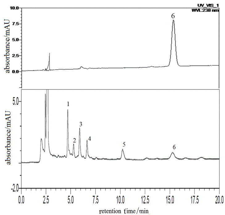
Fig. S1 HPLC chromatography before and after degradation
