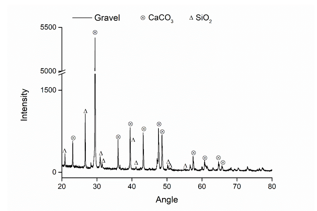
Fig. S2 XRD pattern of the gravel
