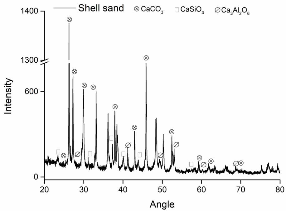
Fig. S3 XRD pattern of the shell sand
