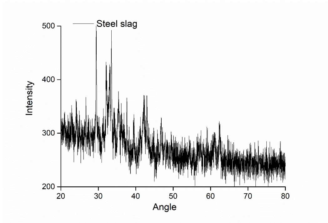
Fig. S1 XRD pattern of the steel slag
