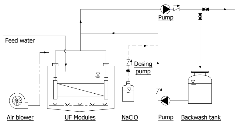
Fig. S1 Schematic diagram of ultrafiltration membrane filtration system
