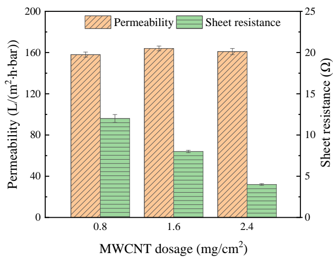
Figure S1. Water permeabilities and sheet resistances of PVDF supported CNT membranes with different CNT dosages. (Sheet resistance is a measure of the electric resistance of thin films.)
