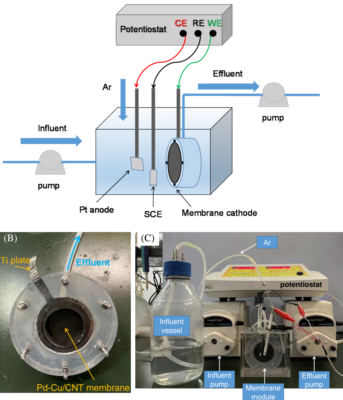
Figure S2. (A) Schematic diagram of the three-electrode filtration cell, (B) photograph of the membrane module and (C) photograph of the flow-through system.
