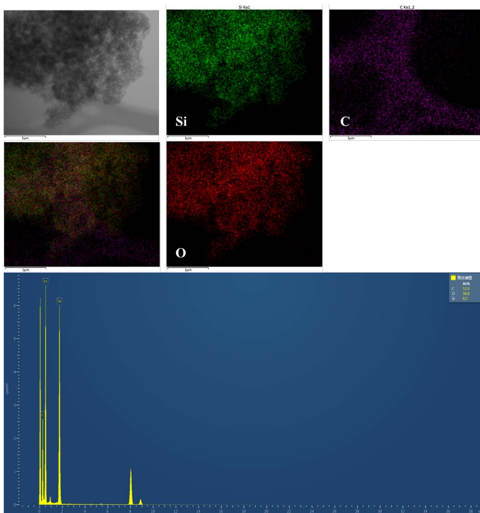
Fig. S2 EDS spectra of “CTAB-0.00”.
