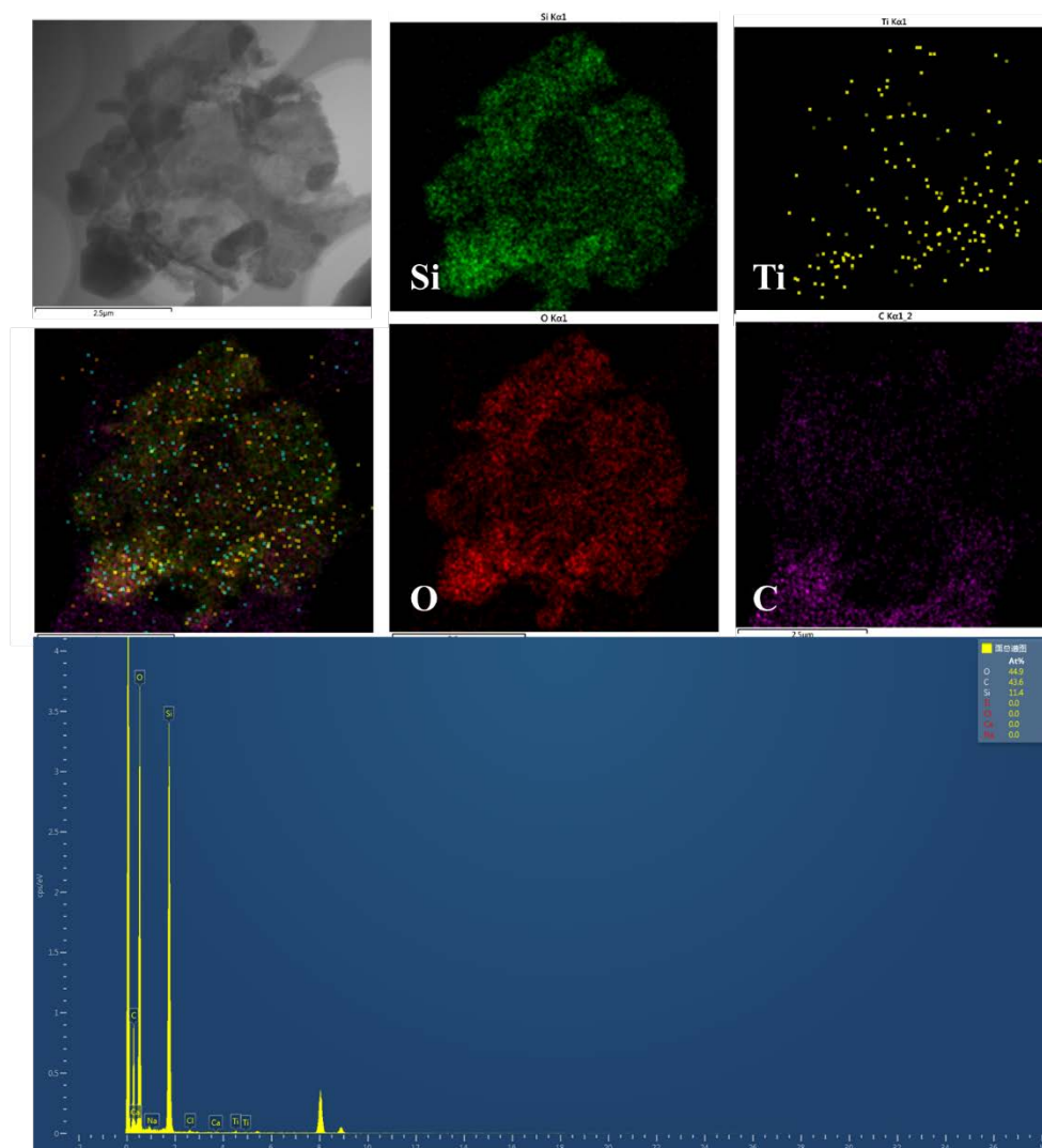
Fig. S3 EDS spectra of “CTAB-0.24”.
