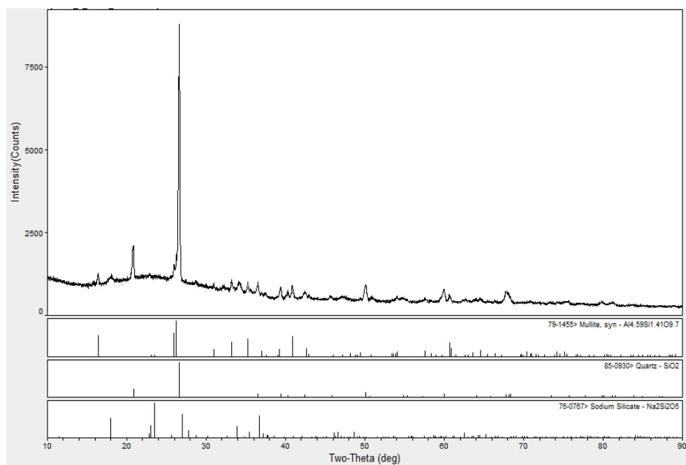
Fig. S1 XRD patterns of the CFA samples used in this work.
