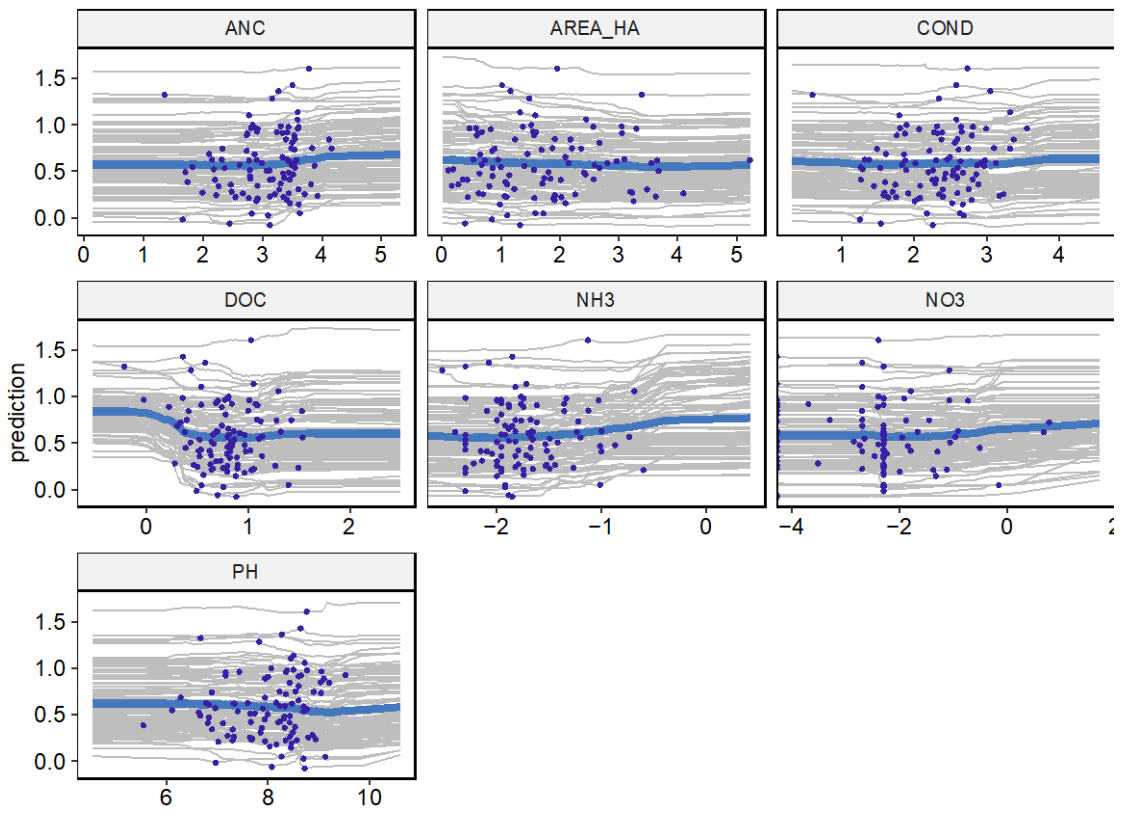
Figure S3 Partial dependence profiles showing changes of potential predictions with acid neutralizing capacity (ANC), lake area (AREA_HA), conductivity (COND), dissolved organic carbon (DOC), ammonia nitrogen (NH 3 ), nitrate nitrogen (NO 3 ), and pH(PH).
