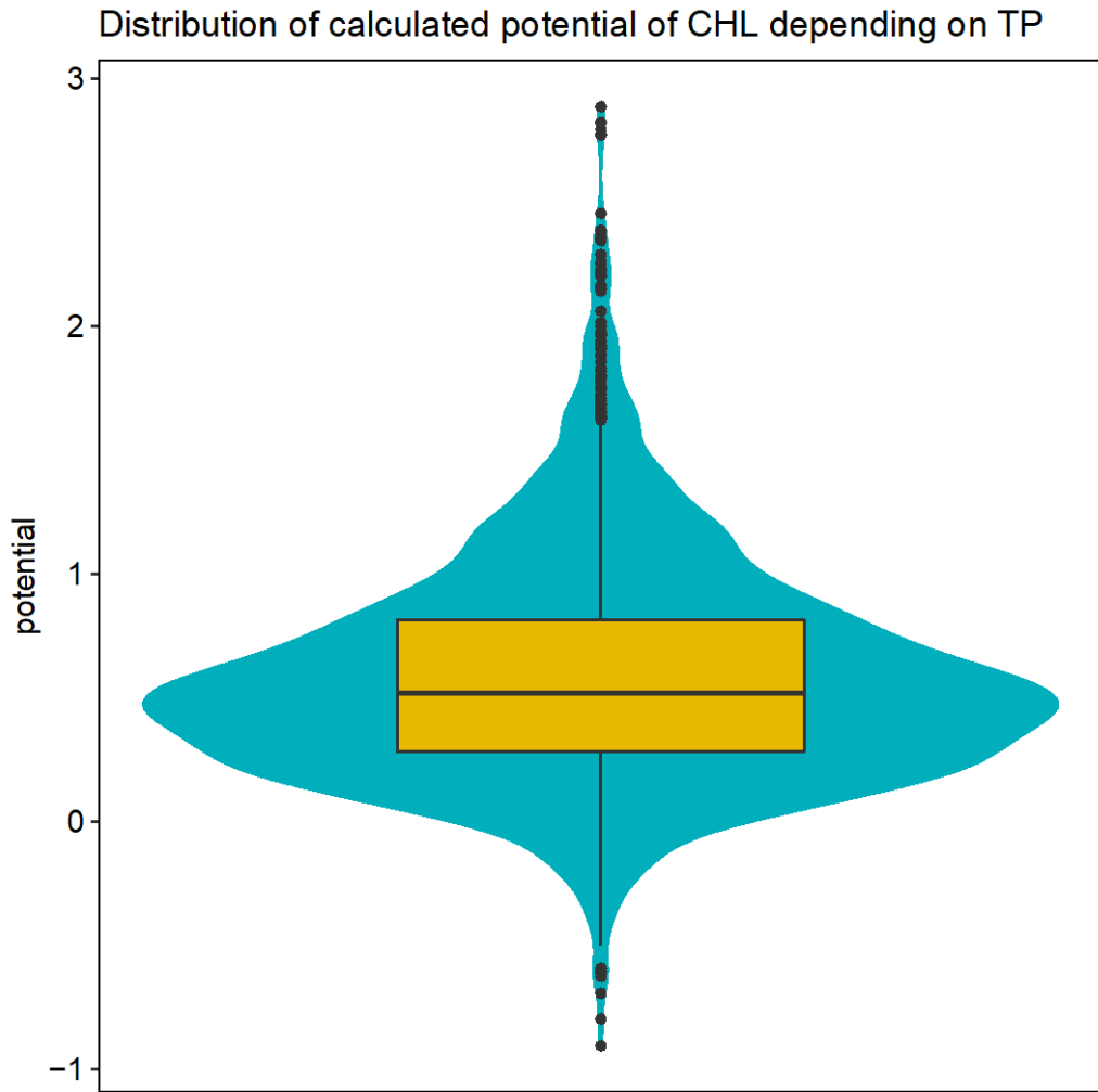
Figure S1 Distribution of calculated potential of CHL depending on TP
