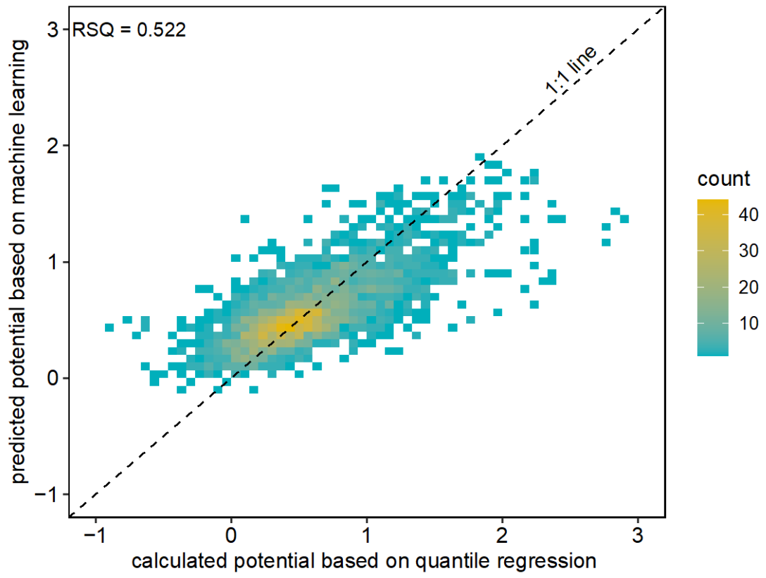
Figure S2 Fitness plot of potential
