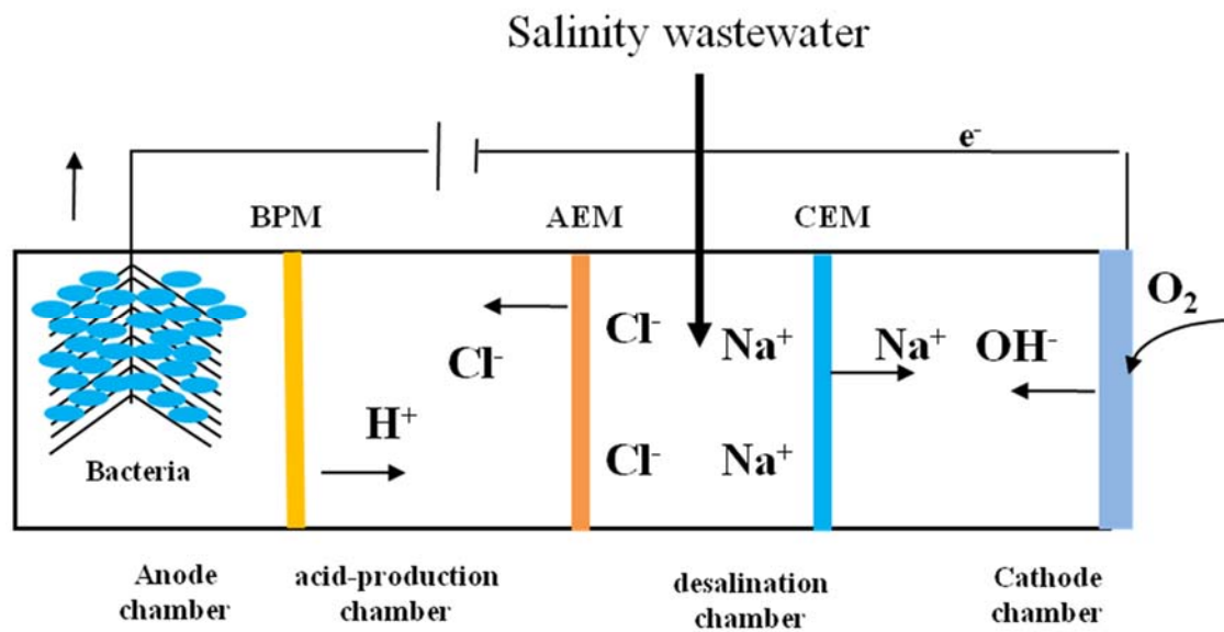
Fig. S1 The schematic diagram of microbial electrolysis desalination and chemical-production cell (MEDCC)
