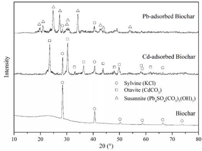
Fig. S1 XRD patterns of corn straw biochar before and after adsorbing Cd and Pb
