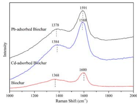
Fig. S4 Raman spectrum of corn straw biochar before and after adsorbing Cd and Pb
