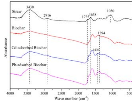
Fig. S3 FTIR spectra of straw and biochar before and after adsorbing Cd and Pb
