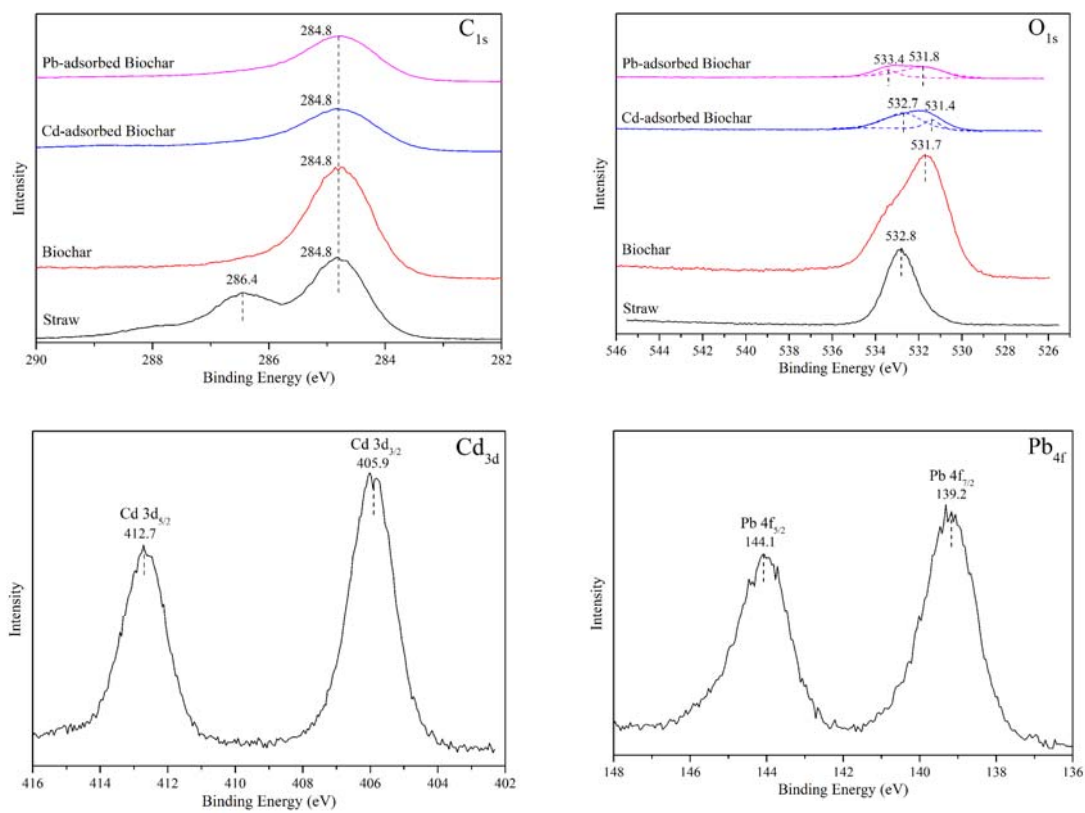
Fig. S2 XPS spectra of C 1s (a), O 1s (b) in straw and biochar before and after adsorbing Cd and Pb, Cd 3d (c) in biochar after adsorbing Cd, Pb 4f (d) in biochar after adsorbing Pb
