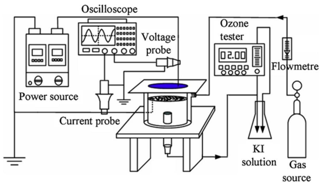
Fig. S1 Experimental setup for soil treatment using non-thermal discharge plasma
