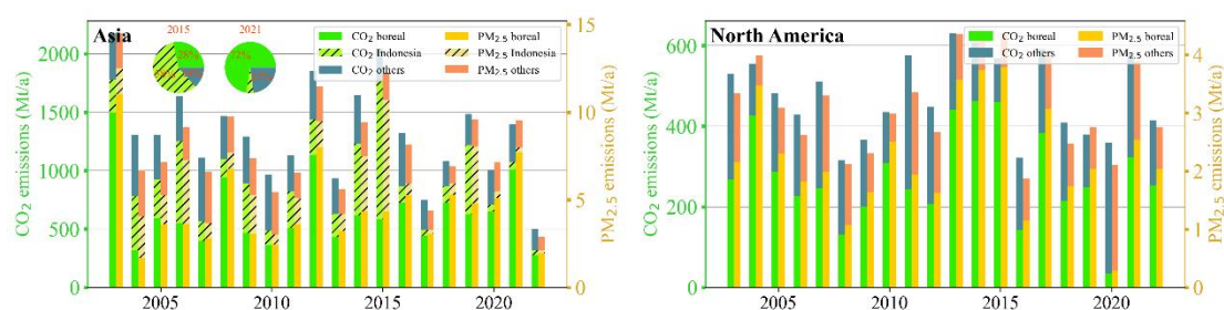
Fig. S2 The emissions of CO 2 (green) and PM 2.5 (orange) in Asia and North America. The stacked bars indicate the Asian emissions contribution from boreal Asia, Indonesia and the rest of Asia and North American emissions contribution from boreal North America and the rest of North America. The inset pie charts for Asia indicate the sources of its CO 2 emissions contribution in 2015 and 2021. Typical El Niño years include 2004, 2006, 2009, 2015, and 2019.
