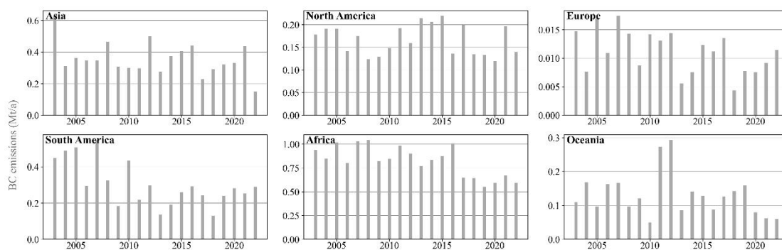
Fig. S1 The emissions of BC (million tons/year) across Asia, North America, Europe, South America, Africa, and Oceania, respectively, during the period 2003–2022. The gray bars denote emissions of BC.
