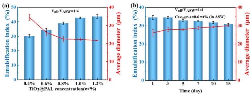
Fig. S2 (a) Effect of TiO_2@PAL concentration on its Pickering emulsification in ASW. (b) The time stability of diesel-in-ASW emulsion stabilized by TiO_2@PAL
