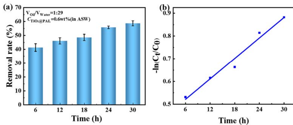
Fig. S3 (a) Removal rate of diesel under different irradiation time in ASW. (b) The fitting curve of -\ln(C_t/C_0) versus time
