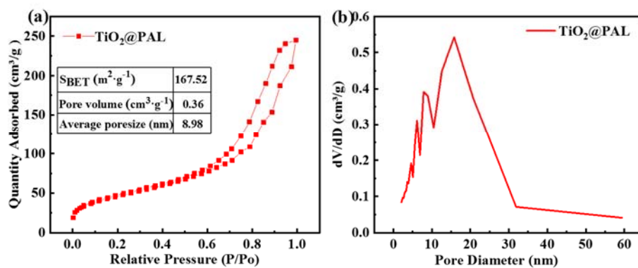
Fig. S1 (a, b) N_2 sorption isotherm and pore size distribution of TiO_2@PAL
