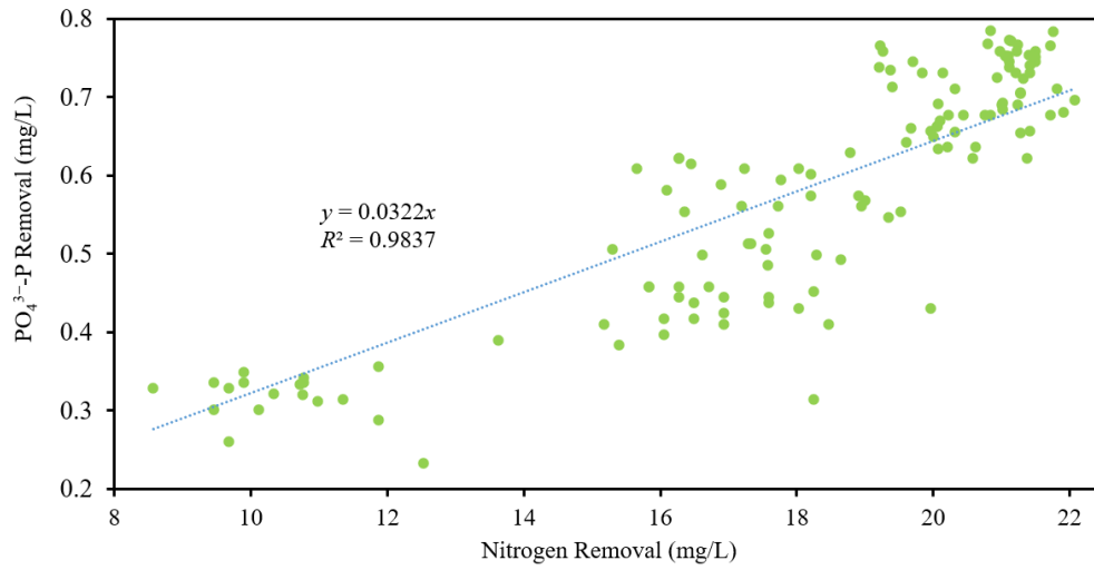
Fig. S3 Positive linear correlation between nitrogen and phosphate removal during the experimental periods.
