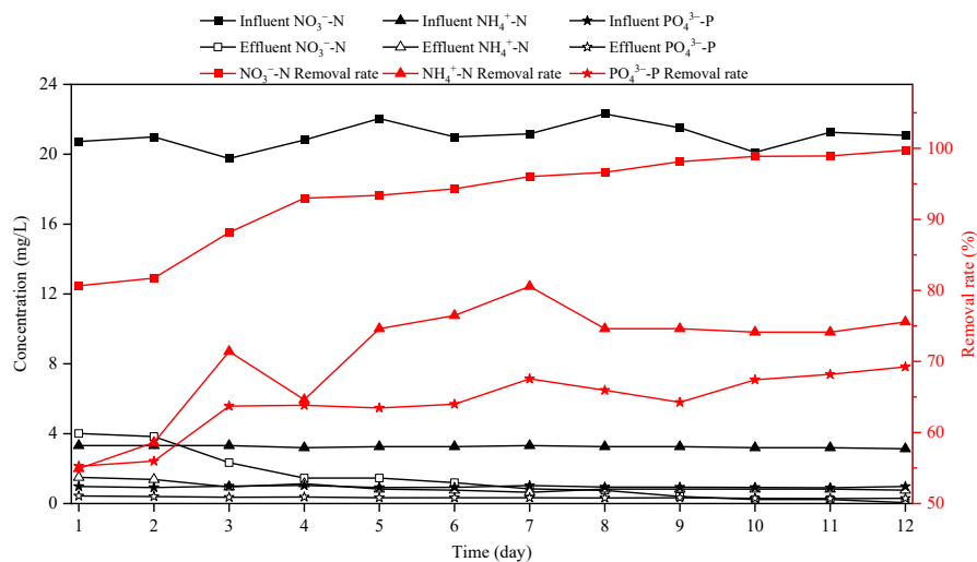
Fig. S1 Profiles of influent/effluent \text{NO}_3^- -N, \text{NH}_4^+ -N, \text{PO}_4^{3-} -P concentration and their removal rate during the start-up of the CGSAD reactor.
