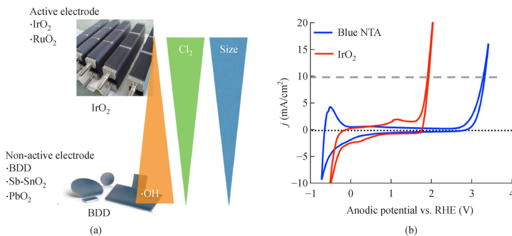
Fig. 2 (a) Classification and properties of active and non-active anodes. (b) Cyclic voltammetry analysis of electrodes in 30 \text{ mmol/L Na}_2\text{SO}_4 electrolyte. \text{IrO}_2 and blue \text{TiO}_{2-x} nanotube array (NTA) represent active and non-active electrodes, respectively. Data was collected from reference (Yang and Hoffmann, 2016).
