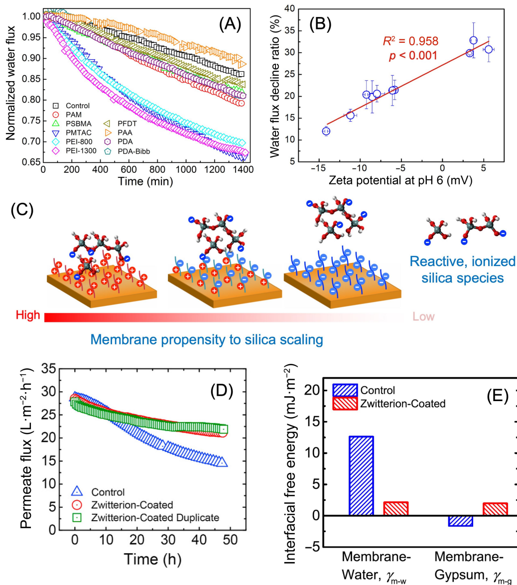
Fig. 5 (A) Water flux curve of RO desalinating feedwater containing supersaturated silica using membranes of different surface properties. (B) The water flux decline ratio of membranes shown in Fig. 5(A) demonstrates a strong correlation with surface charge, manifested by zeta potential, of the membranes. (C) Mechanisms underlying the relationship between membrane surface charge and propensity of silica scaling. (D) Water flux curve of RO desalinating feedwater containing supersaturated gypsum using a pristine polyamide membrane and membranes coated with zwitterionic polymer. (E) The membrane-water and membrane-gypsum interfacial free energies for the pristine polyamide and zwitterion-coated membranes. The figures are adapted with permission from Tong et al. (2017), copyright American Chemical Society; Jaramillo et al. (2021), copyright Elsevier.
