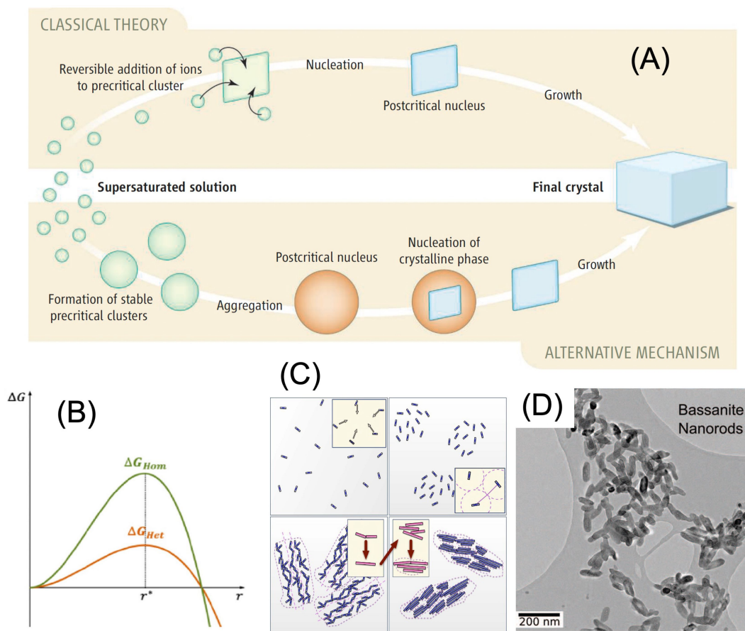
Fig. 1 (A) Schematic of classical nucleation theory and non-classical nucleation pathway of mineral formation. (B) The change of free energy during mineral nucleation. \Delta G_{Hom} and \Delta G_{Het} refer to the free energy barrier to homogeneous nucleation and heterogeneous nucleation, respectively. (C) Schematic of four stages of gypsum crystal formation, including the formation, aggregation, self-assembly, and coalescence of CaSO 4 clusters. (D) Transmission electron microscopic image of bassanite nanorods formed before gypsum crystal formation. The figures are adapted with permission from Meldrum and Sear (2008), copyright American Association for the Advancement of Science; Tong et al. (2019a), copyright Elsevier; Stawski et al. (2016), copyright Nature Portfolio; Van Driessche et al. (2012), copyright American Association for the Advancement of Science.
