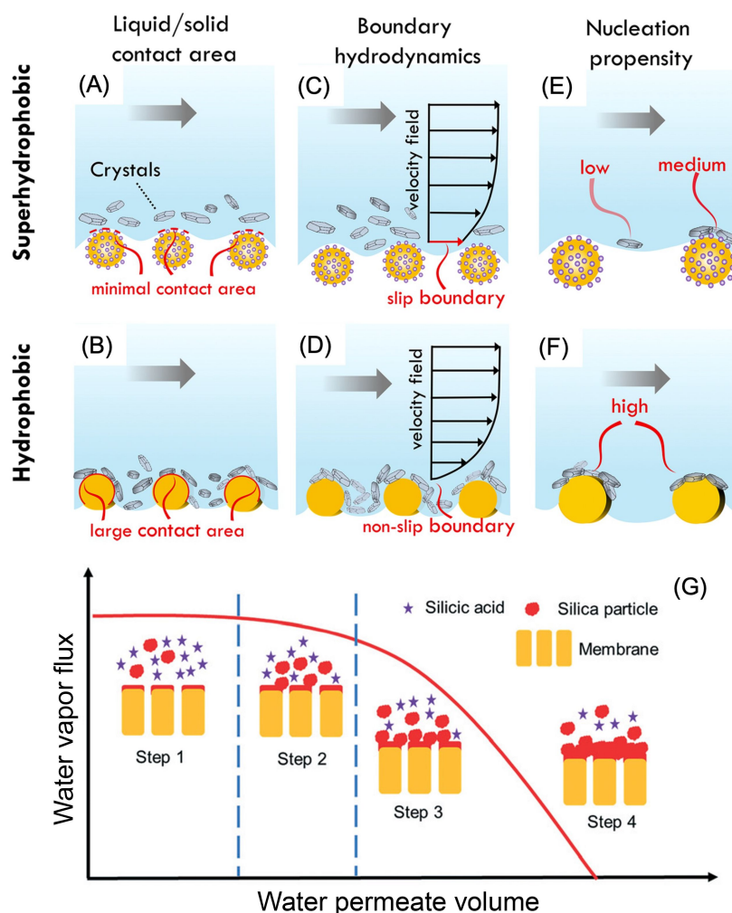
Fig. 6 (A–F) Three possible mechanisms underlying the resistance of superhydrophobic membranes against gypsum scaling in MD. It is worth mentioning that the mechanism shown by Figures 6E and 6F is unlikely to be the main mechanism because gypsum is described more appropriately by a non-classical pathway. (G) A four-step mechanism of silica scaling in MD. The figures are adapted with permission from Horseman et al. (2021), copyright American Chemical Society; Yin et al. (2019), copyright Royal Society of Chemistry.
