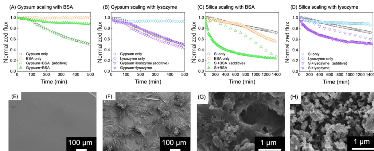
Fig. 4 Representative normalized water flux decline curves for (A and B) gypsum and (C and D) silica scaling in the presence of proteins in RO. Each graph includes water flux curves of individual mineral scaling and organic fouling, the additive curve of individual scaling and fouling, and the actual water flux curve of combined scaling and fouling. (E and F) SEM images of the membrane surface after combined scaling and fouling experiments: gypsum scaling with (E) BSA and (F) lysozyme fouling, and silica scaling with (G) BSA and (H) lysozyme fouling. The figures are adapted with permission from Park et al. (2024) (A, B, E, F), copyright Elsevier; Quay et al. (2018) (C, D, G, H), copyright American Chemical Society.
