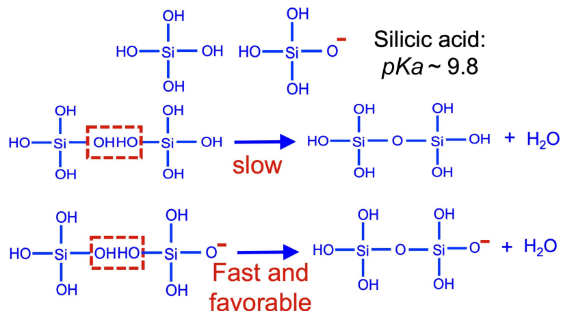
Fig. 2 Schematic of silicic acid polymerization that leads to silica formation.
