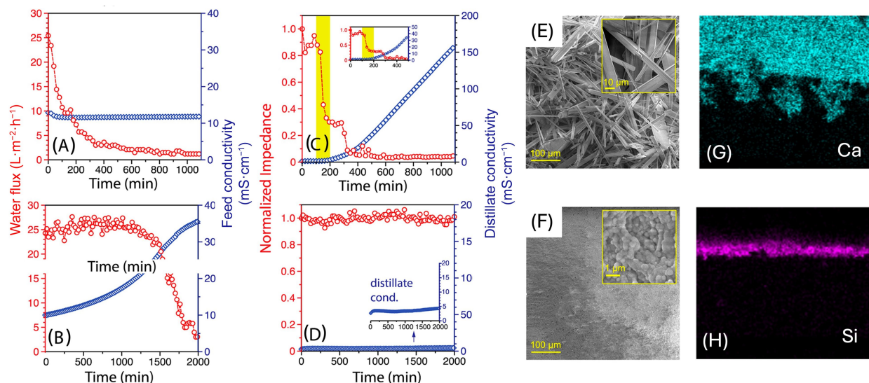
Fig. 3 (A and B) Water vapor flux (red) and feed conductivity (blue) curves during MD desalination in the presence of (A) gypsum scaling and (B) silica scaling. (C and D) Normalized transmembrane impedance (red) and distillate conductivity (blue) during MD desalination in the presence of (C) gypsum scaling and (D) silica scaling. A decrease of normalized impedance and an increase of distillate conductivity indicate the occurrence of pore wetting. (E and F) Top-down SEM images of (E) gypsum and (F) silica scales formed in MD. (G and H) Cross-section energy dispersive X-ray spectroscopy mapping of membranes scaled by (G) gypsum and (H) silica. The figures are adapted with permission from Christie et al. (2020) , copyright American Chemical Society.
