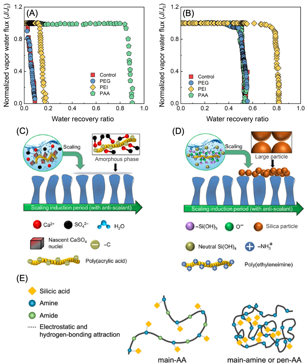
Fig. 7 (A and B) Normalized water vapor flux as a function of water recovery in MD for (A) gypsum scaling and (B) silica scaling in the presence of different antiscalant candidates. (C and D) Schematic illustration of the mechanisms of antiscalants for mitigating (C) gypsum scaling and (D) silica scaling in MD. (E) Schematic illustration of amino-containing polymers of different conformation hindering silica polymerization through interactions with silicic acid. The figures are adapted with permission from Yin et al. (2021), copyright American Chemical Society; Kaneda et al. (2024), copyright American Chemical Society.
