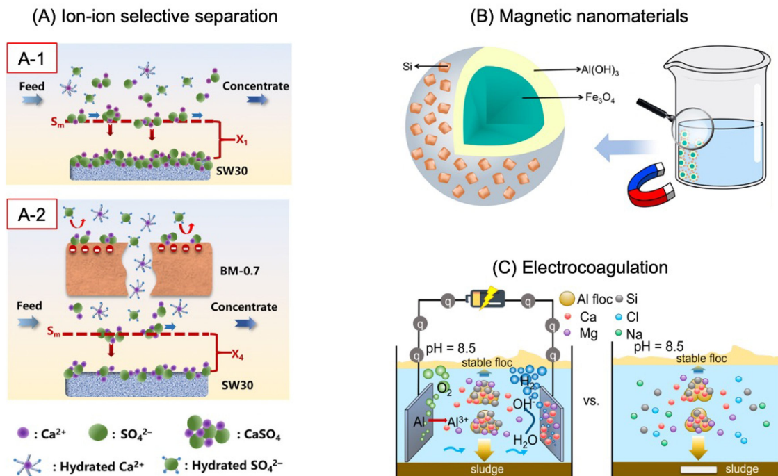
Fig. 8 Schematic illustrations of different pretreatment techniques. (A) Ion-ion selective separation process using NF for gypsum scaling mitigation. (B) Magnetic iron-aluminum hybrid nanomaterials for silica removal. (C) Electrocoagulation for removing silica and hardness. The figures are adapted with permission from (Zhang and Zhang, 2021) (copyright Elsevier), (Guan et al., 2019) (copyright American Chemical Society) and (Liu et al., 2022) (copyright American Chemical Society).
