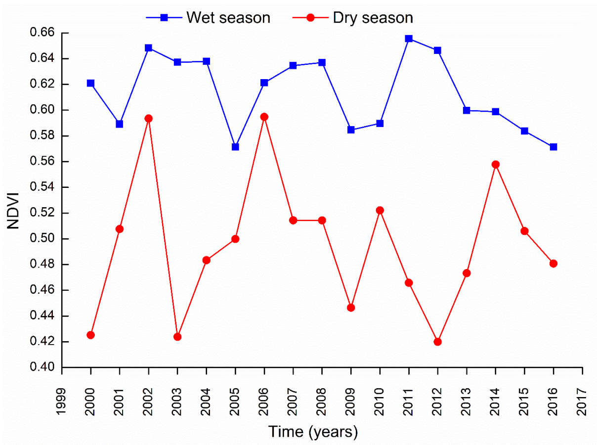
Supplementary Fig. S1: NDVI variation between wet season and dry season from 2000 to 2016
