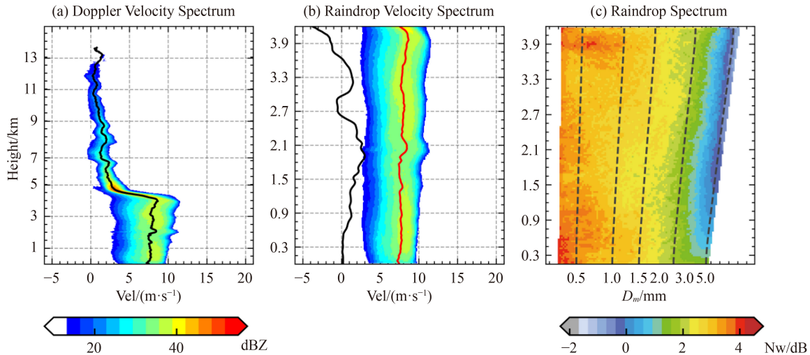
Fig. 3 Profiles of reflectivity factor-weighted Doppler velocity spectral densities [ 10 \log(\text{mm}^6 \cdot \text{m}^{-3} (\text{m} \cdot \text{s}^{-1})^{-1}) ] at 08:22:40 LCT on June 6, 2020. (a) Doppler velocity spectrum, (b) Raindrop Velocity Spectrum removed Vair (Vair with black line and mean fall speed with red line), and (c) Raindrop Spectrum.
