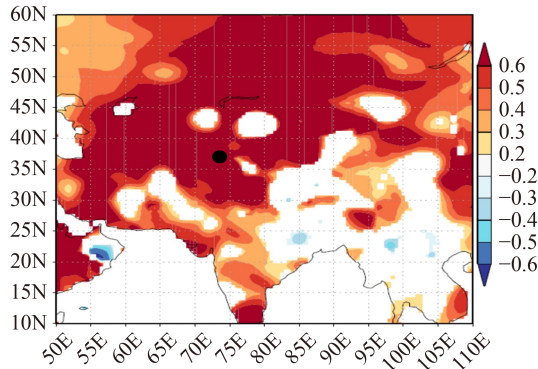
Fig. 6 Spatial correlation field of reconstructed June–July mean temperatures with gridded mean temperature from the CRU TS 4.05 data set 1955–2013. Correlation analysis was performed using the KNMI climate explorer. Black circle is the sampling site in the Himalayas northern Pakistan. Correlations are not shown if significant level p > 0.05 .
