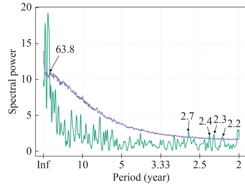
Fig. 7 Multi-taper spectrum of our temperature reconstruction and confidence intervals of 95%.
