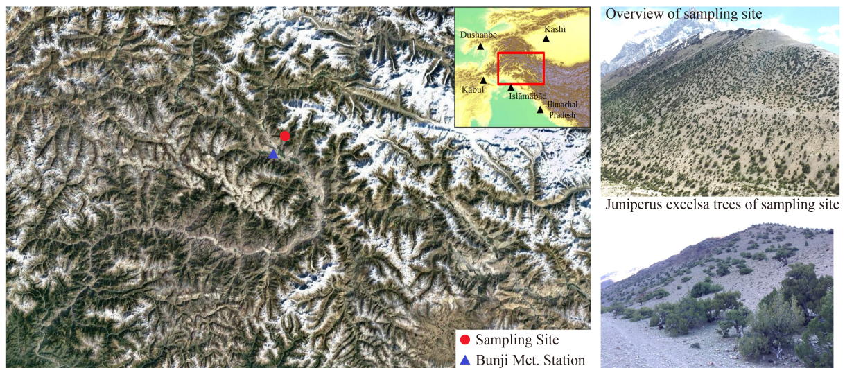
Fig. 1 Tree-ring sampling site, meteorological station and overview of the sampling area used in this study.
