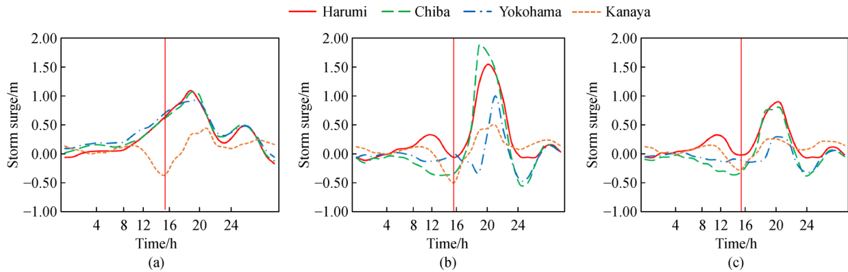
Fig. 10 Storm surge hydrographs generated for (a) original Typhoon Lan, (b) 50% increase in Typhoon Lan wind speed, and (c) 50% decrease in Typhoon Lan wind speed. The red vertical lines indicate time of landfall.
