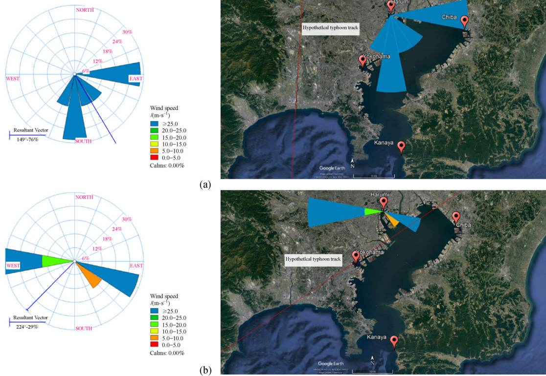
Fig. 5 Simulated wind diagram at landfall for the Harumi observation station during passage of typhoon (a) Case A-11 (landfall location 25 km southwest of Tokyo Bay, \theta = 90^\circ ); (b) Case A-13 (landfall location 25 km southwest of Tokyo Bay, \theta = 150^\circ ).
