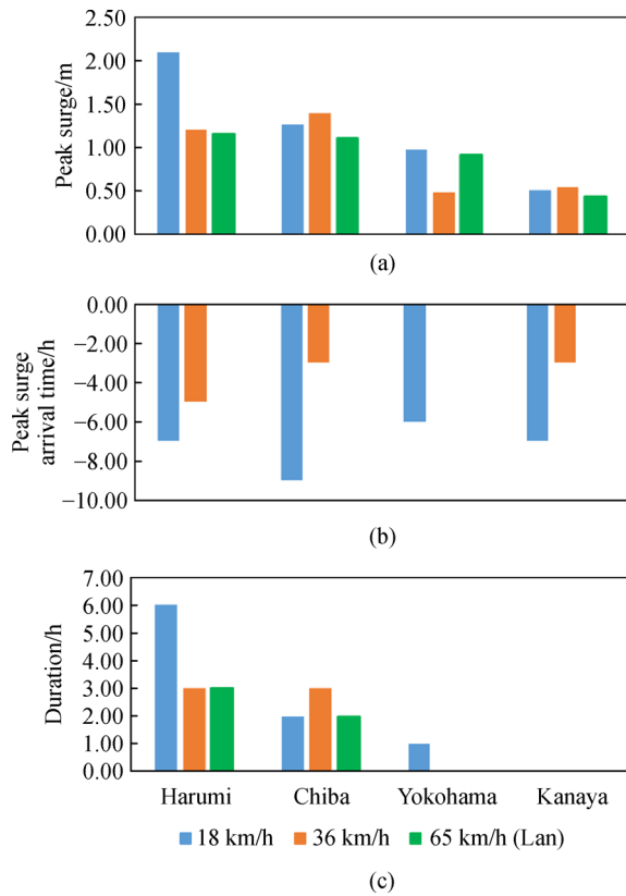
Fig. 6 Comparison of (a) peak storm surge, (b) peak surge arrival time, and (c) duration of storm surge over 1 m for typhoons with different forward speeds. Note, the arriving times in (b) and higher surge durations in (c) are relative to those observed during the actual passage of Typhoon Lan.
