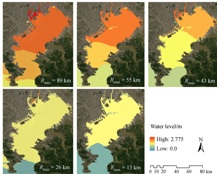
Fig. 9 Distribution of simulated water level during the passage of Typhoon Lan over Tokyo Bay varying with R_{max} .
