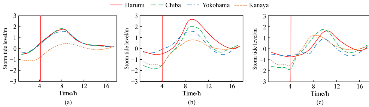
Fig. 4 Comparison of storm tide level for selected sets of landfall locations and approach angles: (a) original landfall (OL; 140° approach angle), (b) 100 km east of OL and 90° approach angle (Case A-11), and (c) 150 km east of OL and 90° approach angle (Case A-18). The red vertical lines indicate time of typhoon landfall.
