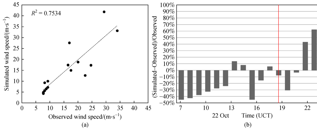
Fig. 2 (a) Simulated vs. observed wind speed at Haneda, Tokyo, and (b) estimated wind speed error. The red vertical line indicates the time of landfall of Typhoon Lan (2017).
