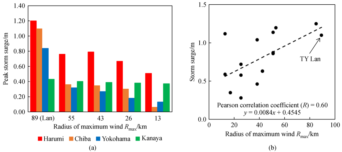
Fig. 8 (a) Comparison of peak storm surge height (in m) for typhoons of different size (in terms of R_{max} ) and (b) observed peak storm surge (JMA, 2019c) vs. typhoon size ( R_{max} ) at typhoon landfall at the Harumi observation station during 1979–2018. The dashed line shows the correlation gradient between the observed storm surge and R_{max} .
