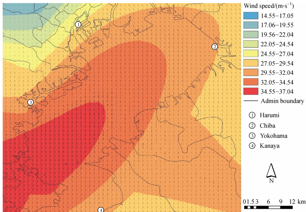
Fig. 7 Wind speed and direction during peak surge at Harumi for typhoon forward speed of 18 km/h
