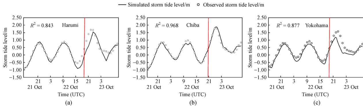
Fig. 3 Comparison of observed and simulated storm tide at (a) Harumi, (b) Chiba, and (c) Yokohama. The red vertical lines indicate the time of landfall of Typhoon Lan (2017).
