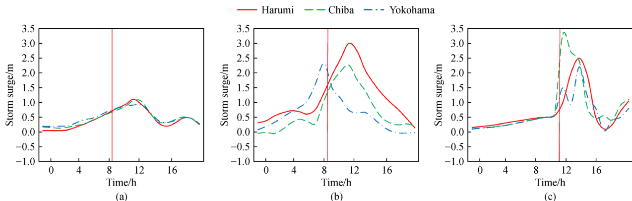
Fig. 11 Comparison of storm surge heights due to (a) Typhoon Lan; (b) a hypothetical typhoon (landfall location 25 km southwest of Tokyo Bay, \theta = 100^\circ , forward speed of 18 km/h, R_{\max} = 89 km, Lan intensity increased by 50%); and (c) the hypothetical typhoon assumed by Ministry of Land, Infrastructure, Transport and Tourism (MLIT) (landfall location 25 km southwest of Tokyo Bay, \theta = 100^\circ , forward speed of 50 km/h, intensity of 915 hPa at landfall time, sea level rise of 0.6 m due to global warming). The red vertical lines indicate time of landfall.
