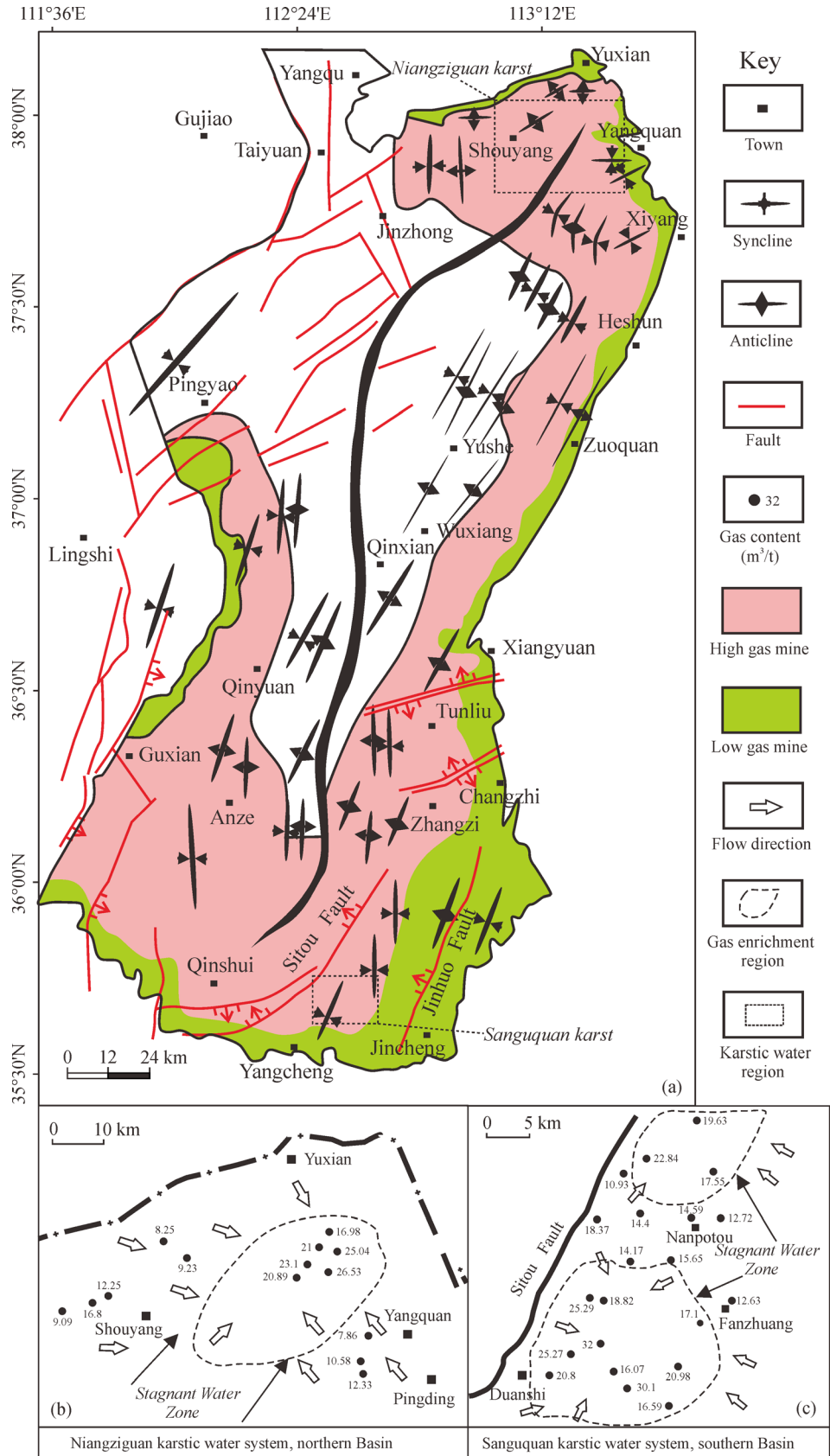
Fig. 1 (a) The tectonic outline map with the distribution of mine gas grade in the Qinshui Basin; (b) the changes of gas content close to the Niangziguan karstic groundwater system in the northern basin; (c) the variation of gas content close to the Sanguquan karstic groundwater system in the southern basin; gas content data from Song et al. (2013).
