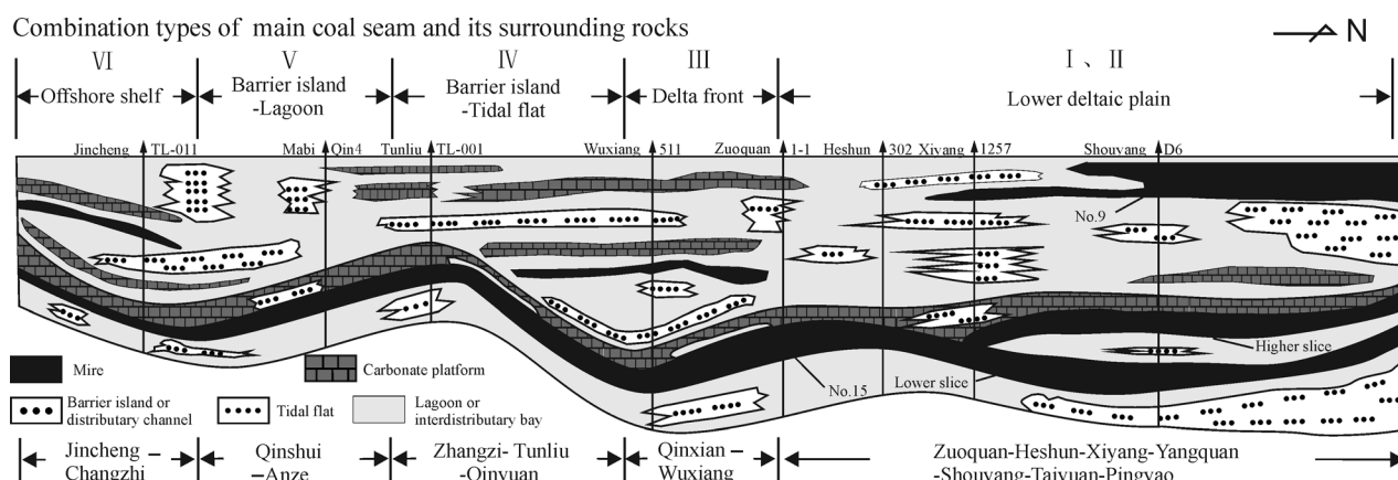
Fig. 8 Sedimentary facies and surrounding rocks of coal measures in the Taiyuan Formation, Qinshui Basin.
