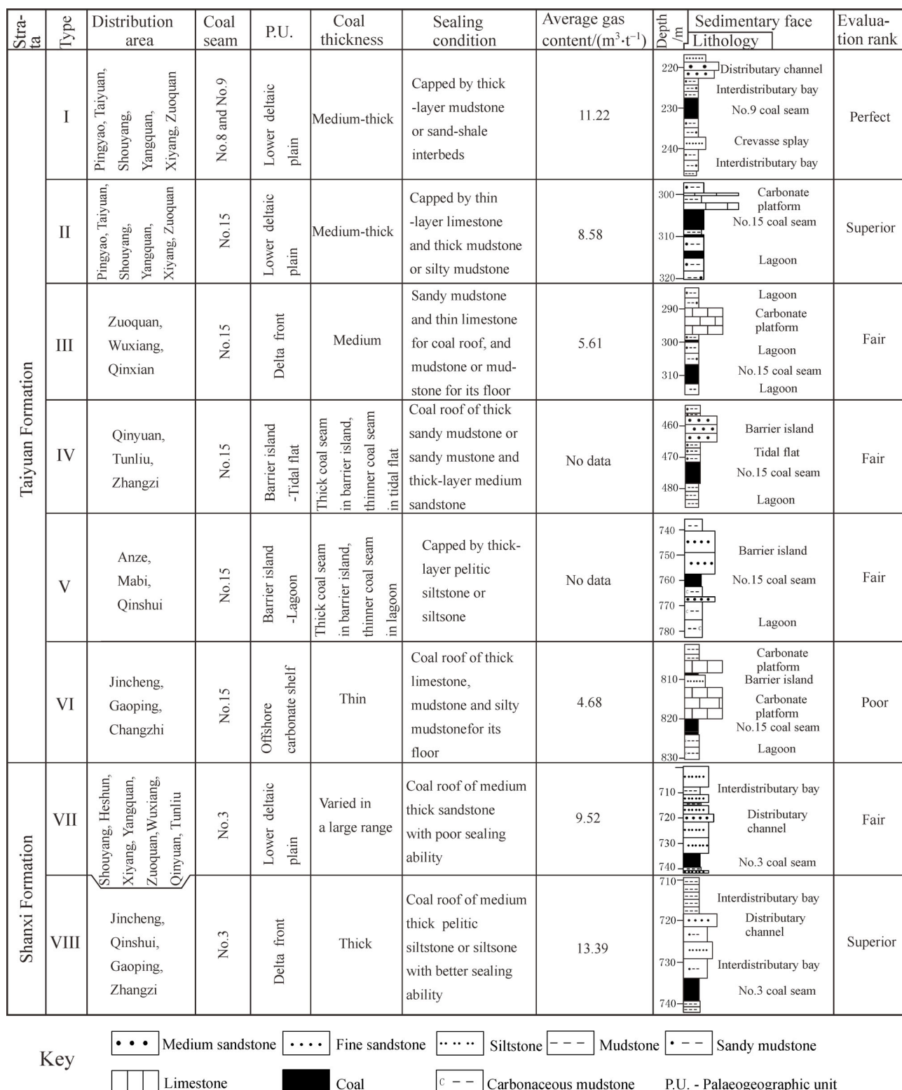
Fig. 10 Types of main coal seam surrounding rock combinations and gas bearing evaluation of the Taiyuan and Shanxi coals in the Qinshui Basin.
