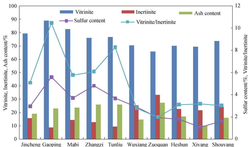
Fig. 7 The coal macerals and coal qualities of No. 3 coal seam of the Shanxi Formation in the Qinshui Basin.
