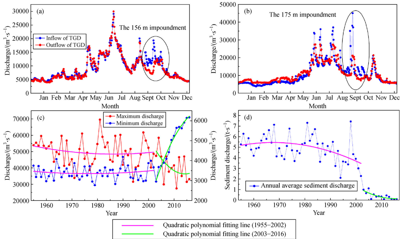
Fig. 4 Variations in discharge and sediment before and after the operation of the TGD. (a) and (b) The inflow and outflow of TGD in 2006 and 2011, respectively; (c) the maximum and minimum discharges at Yichang during the period from 1955–2016; (d) the sediment discharge at Yichang from 1955 to 2016.
