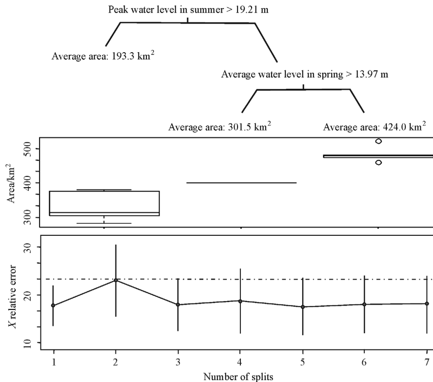
Fig. 9 The final CART model for the coverage area of reeds.
