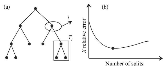
Fig. 4 An example of a CART Tree model (the child node and the sub tree) (a) and the plot of the cross-validated deviance versus tree size for pruning a CART tree (b).
