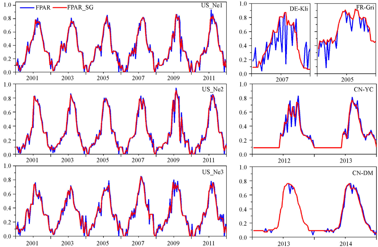
Fig. 4 FPAR and reconstructed FPAR (FPAR_SG) at seven flux sites.
