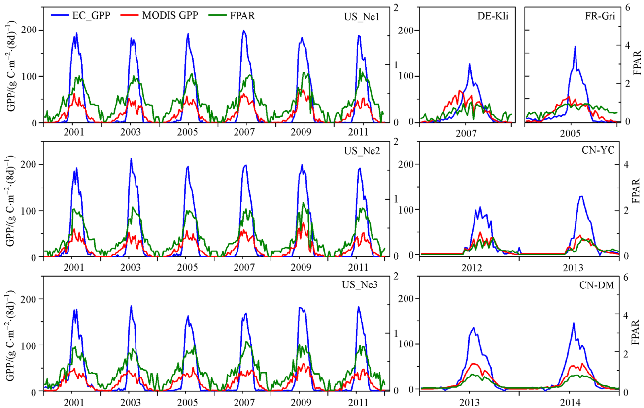
Fig. 5 The relationship between the GPP_{EC} , GPP_{MOD} , and FPAR at seven maize eddy flux tower sites.
