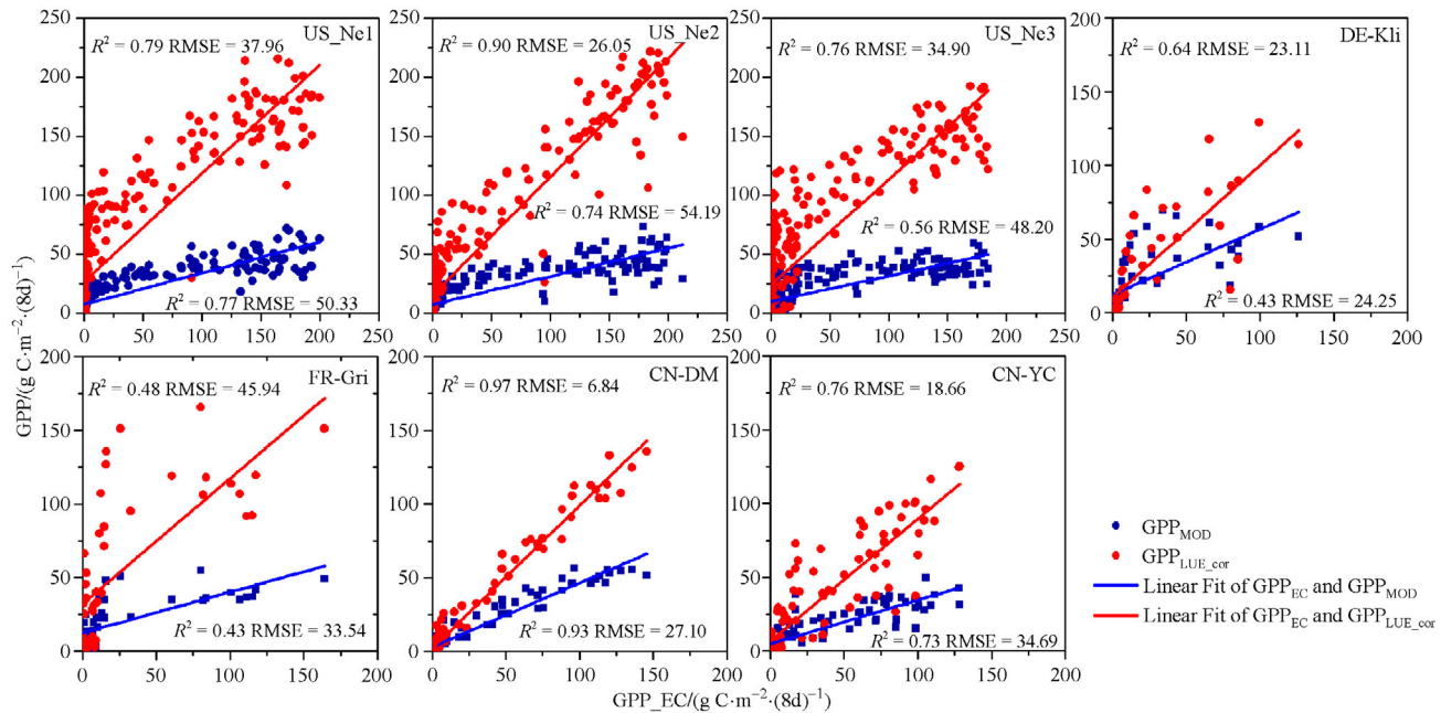
Fig. 3 The scatter plots between GPP_{MOD} , GPP_{LUE\_cor} , and GPP_{EC} at seven maize eddy flux tower sites.
