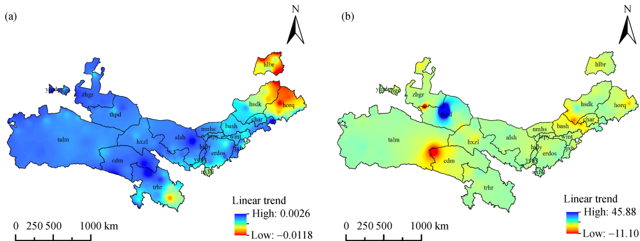
Fig. 6 The linear trend of aridity/humidity index of desertified land of North China from 1981 to 2010.
