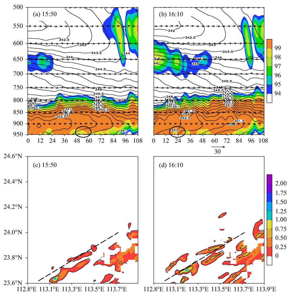
Fig. 11 (a) and (b) Inclined vertical section of equivalent potential temperature (contour lines; unit: K), vertical circulation (arrows; vertical velocity was magnified by 10 times; unit: m·s -1 ) and relative humidity (color shades; unit: %) along the black dashed line shown in Fig. 8. (c) and (d) horizontal distribution of Ri on 900 hPa (color shades; contour lines marking the scope of 0 < Ri < 0.5 ; the black dashed line represents the location of the primary convective line). (a) and (c) represent 15:50, and (b) and (d) represent 16:10.
