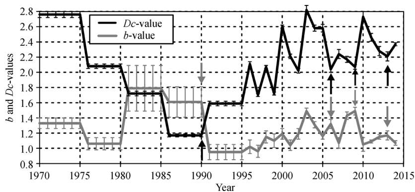
Fig. 11 Changes in two fundamental parameters b and D_c -values from 1970 to 2015 in the Eastern Anatolian Region of Turkey. Arrows show the starting times in decreasing b -values and increasing D_c -values. Standard errors are also shown.
