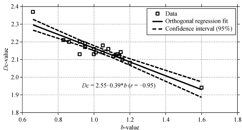
Fig. 9 Estimated orthogonal regression fit for the relationship between b -value and D_c -value. Resulting equation, correlation coefficient, and confidence interval of 95%, for the Eastern Anatolian Region of Turkey are also given. There are 12 events in the confidence interval of 95%.
