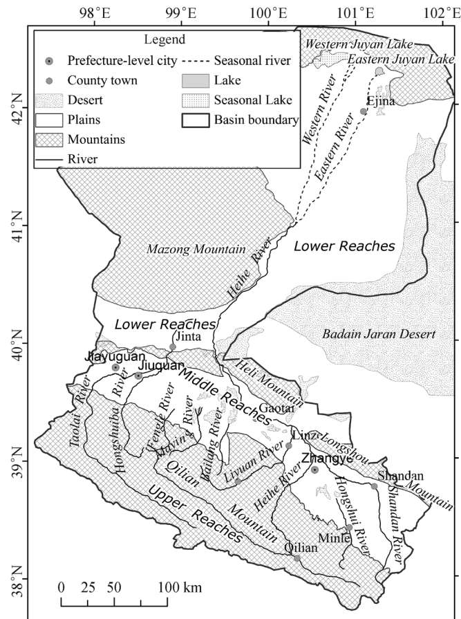
Fig. 1 (a) The location of the HRB locates in northwest China and (b) the HRB origins from the Qilian Mountain, crossing the plains and falls into Juyuan lakes in the north.
