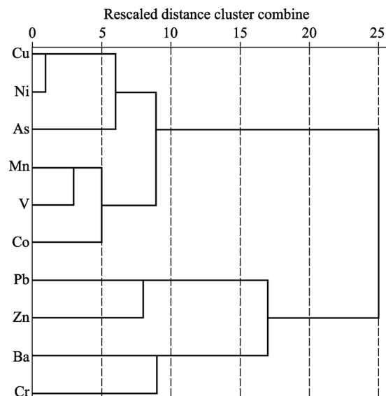
Fig. 3 Dendrogram results of cluster analysis based on Ward method hierarchical cluster analysis for 10 elements.
