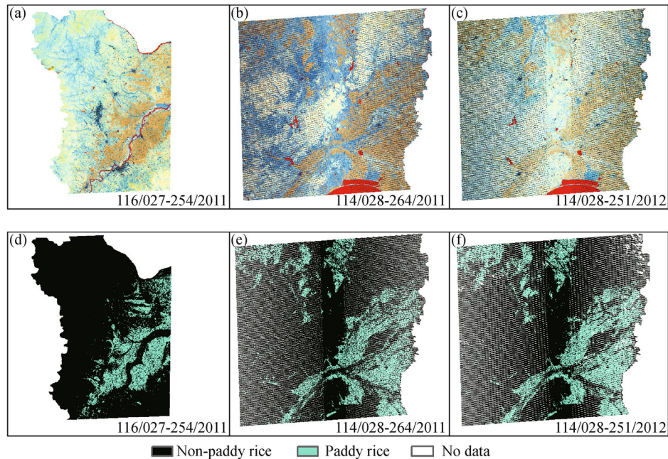
Fig. 7 (a)–(c), Landsat FCC images (R/G/B = LSWI / NDVI / (NDVI + EVI)/2-LSWI); (d)–(f), ripening rice maps for 116/027-254/2011, 114/028-264/2011, and 114/028-251/2012.
