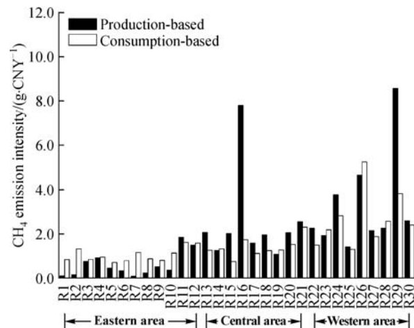
Fig. 11 CH 4 emission intensities by region under different principles in 2007.
