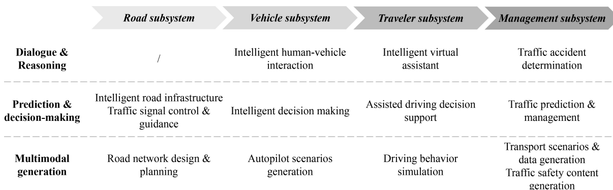
Fig. 2 Integration framework of AIGC and ITS.
