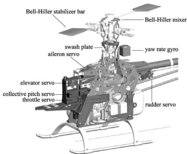
Fig. 3 Typical hardware configuration of single-rotor RC helicopter
