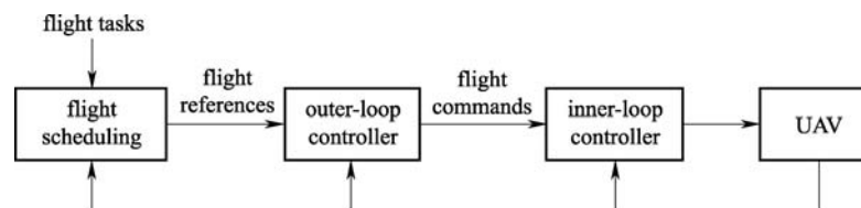
Fig. 10 Structure of overall autonomous flight control
