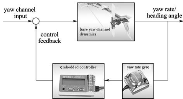
Fig. 4 Configuration of yaw channel in single-rotor RC helicopter
