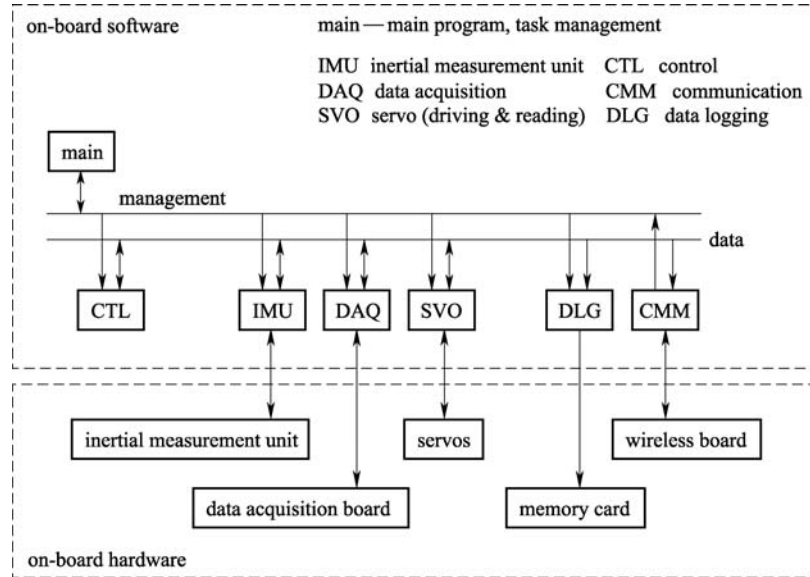
Fig. 8 Framework of an avionic software system
