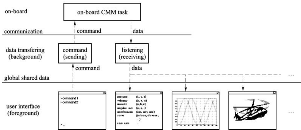
Fig. 9 Framework of ground station software system
