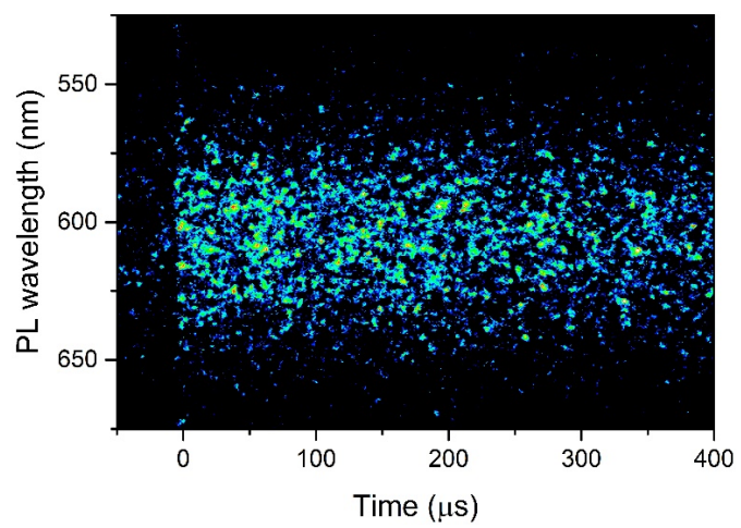
Fig. 2 ESM-2. Time-resolved PL spectrum of the energetically lower PL band of PQD1-PD
