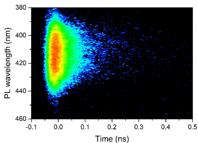
Fig. 1 ESM-1. Time-resolved PL spectrum of the energetically higher PL band of PQD1-CS
