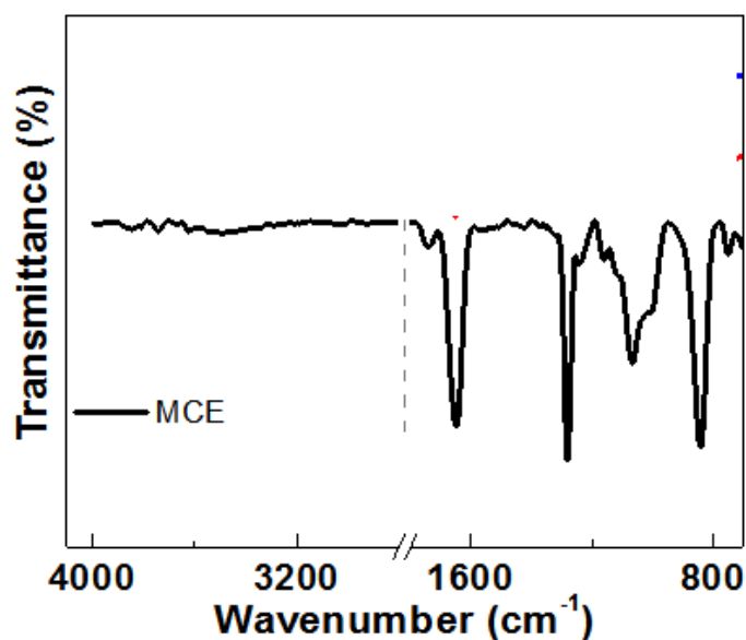
Fig. S1 FTIR spectra of MCE support membrane.
