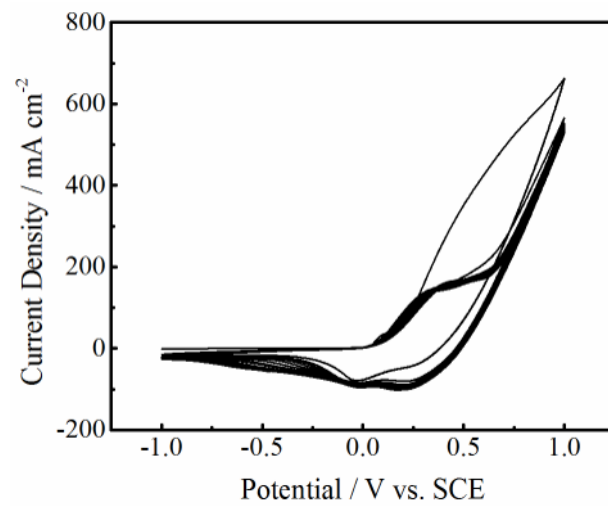
Fig. S3 CV curves of CoHS before data collection in the electrochemical testing.
