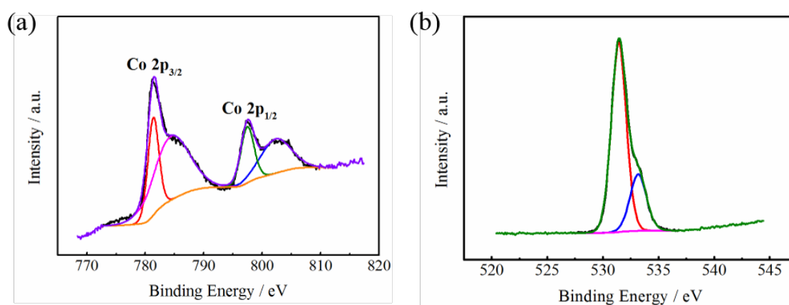
Fig. S2 (a) Co 2p and (b) O 1s of XPS spectra for CoHP.
