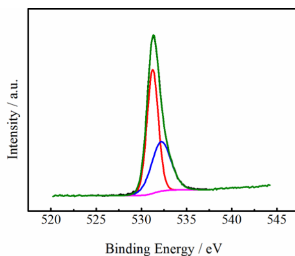
Fig. S1 O 1s XPS spectra of CoHS.
