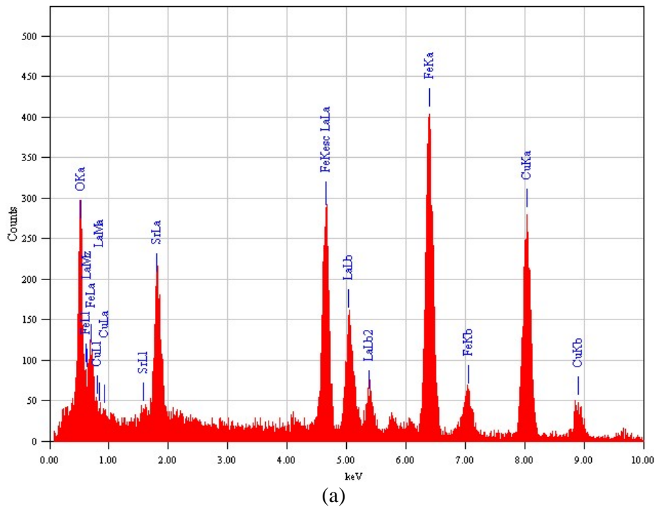
Figure S1: EDS analysis on: a) area marked with “eds1”, b) area marked with “ed4” in aged LSCF + NLC sample image shown in Figure 4d.
