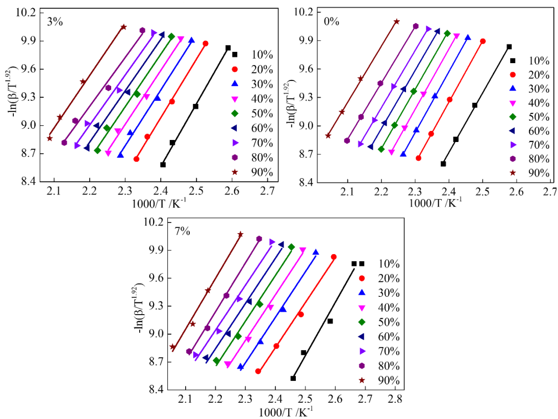
Fig. S4 Relationship between -\ln(\beta/T^{1.92}) versus 1000/T for the investigated samples
