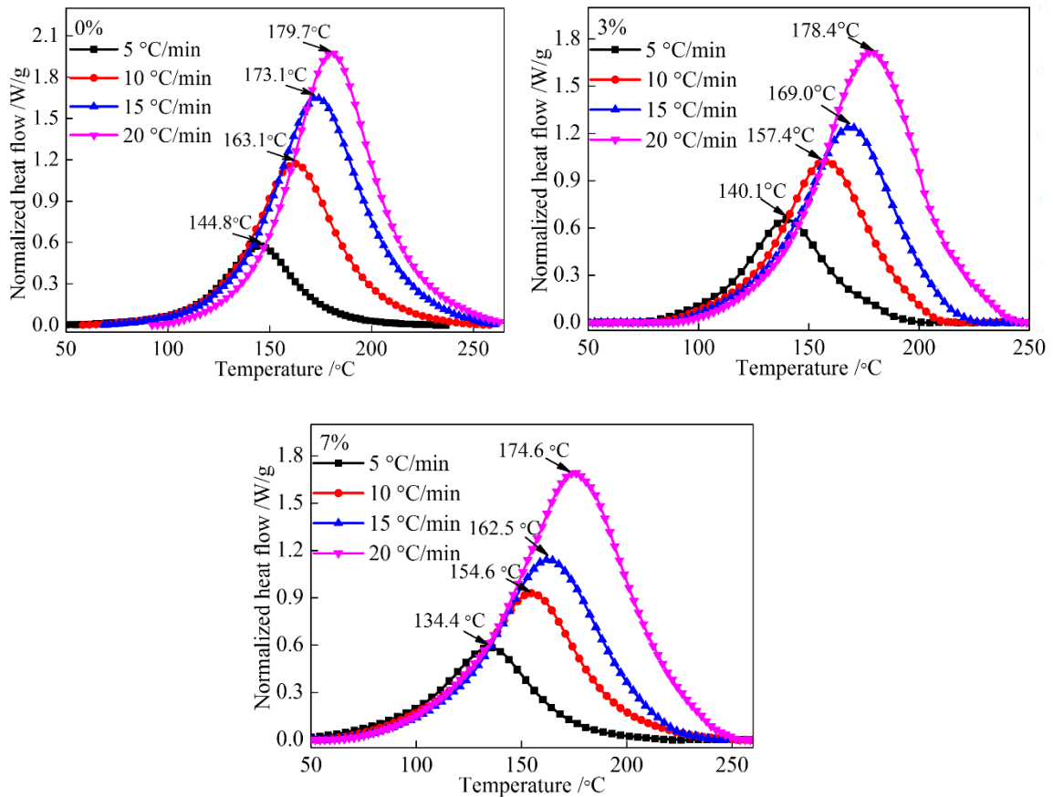
Fig. S2 DSC thermograms of samples with linear-increased heating rates
