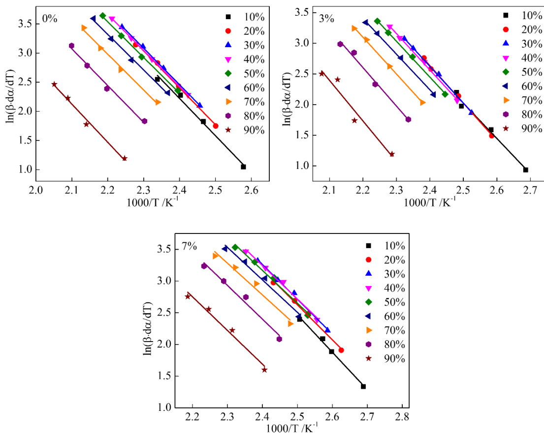
Fig. S3 Plots of \ln(\beta \cdot d\alpha/dT) against 1000/T according to Friedman equation for the investigated samples
