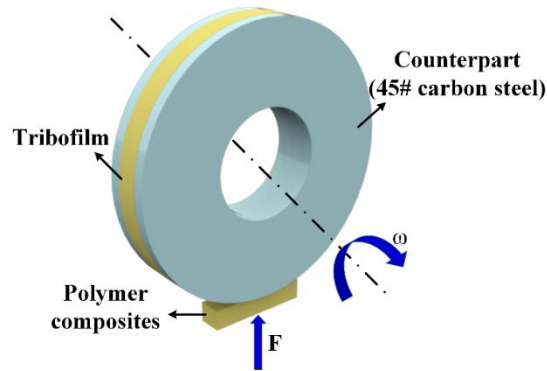
Fig. S1 Schematic drawing of a friction couple during sliding wear testing
