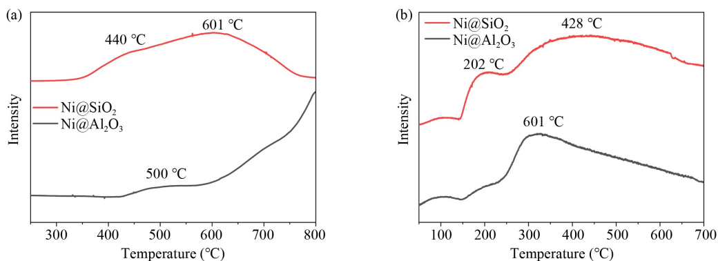
Fig. 8 (a) H 2 -TPR profiles of 20 wt % Ni@ \gamma -Al 2 O 3 and 20 wt % Ni@SiO 2 ; (b) CO 2 -TPD profiles of 20 wt % Ni@ \gamma -Al 2 O 3 and 20 wt % Ni@SiO 2 .
