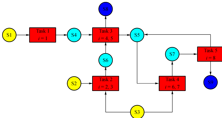
Fig. 1 STN representation of a multipurpose batch process facility (Example 2).
