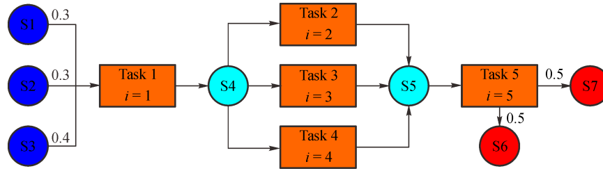
Fig. 14 STN representation of Example 9.
