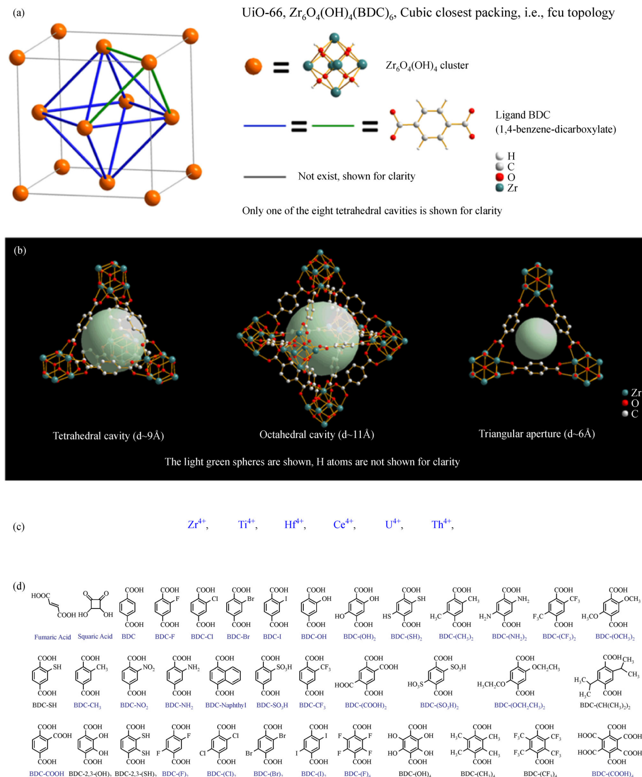
Fig. 1 (a) The unit cell of UiO-66 constructed with \text{Zr}_6 cluster and BDC ligand. (b) The structure of UiO-66 cavities and aperture. The size of cavities and aperture is estimated from the largest spheres which may fit them. (c) Possible tetravalent metal ions for preparing UiO-66 type MOFs. (d) Possible BDC type ligands for constructing UiO-66 type MOFs. Ligands labeled in blue indicate their corresponding MOFs have been reported. Reproduced from [28] and [29] with permissions, copyright American Chemical Society, 2015 and Royal Chemical Society, 2015.
