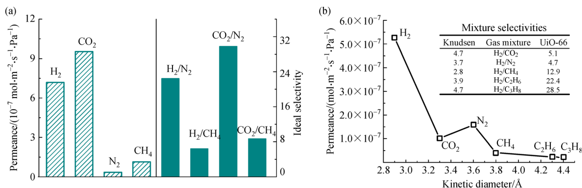
Fig. 7 (a) Single component permeation data of UiO-66 membranes at 293 K with 1 bar pressure difference; (b) H 2 mixed binary permeation data of (002) oriented UiO-66 membrane at 298 K and 1 bar (absolute pressure) in both feed and sweep sides. Reproduced from [28,95] with permissions, copyright American Chemical Society, 2015 and 2017.
