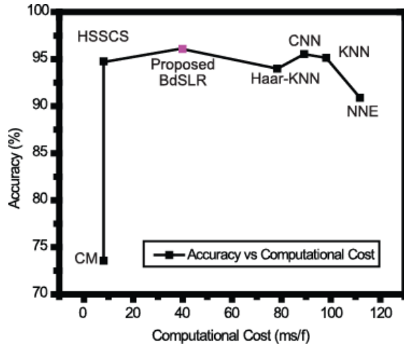
Fig. Comparative analysis of different systems where red color indicates our proposed two-steps classifier based method.
