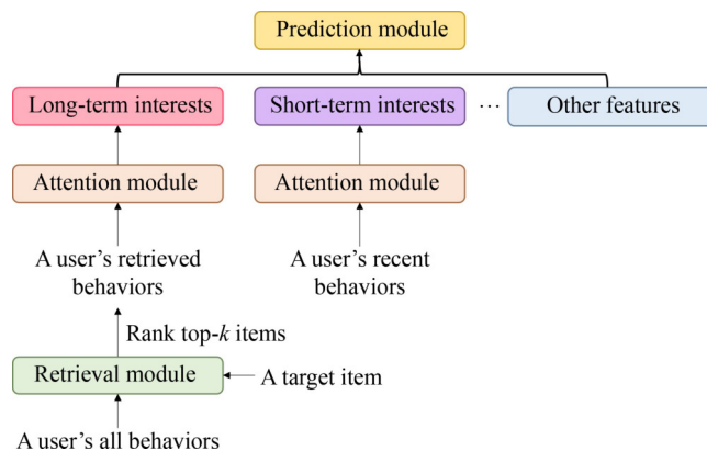
Fig. 13 Illustration of a typical ultra-long sequential recommendation method
