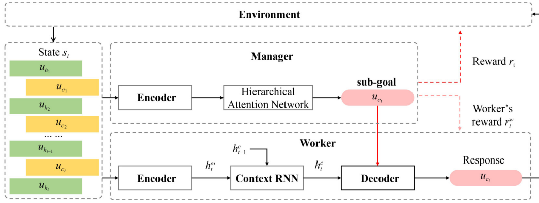
Fig. 4 The overall framework of GoChat [110], which utilizes hierarchical reinforcement learning (HRL) to concurrently plan high-level and low-level policy for efficiently achieving topic path planning
