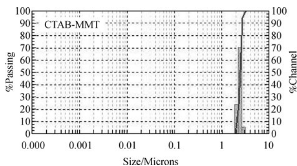
Figure 8 Zeta particle analysis of CTAB modified MMT
