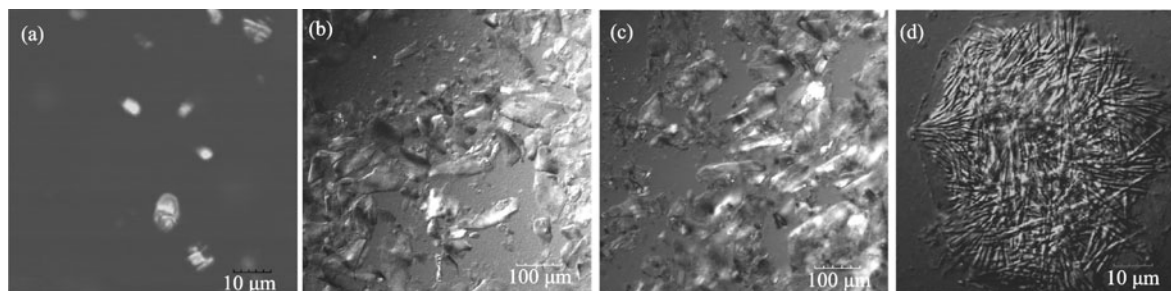
Figure 5 Micro image of the gels (Zn- 1a ) with concentration of (a) 10, (b) 20, (c) 40, and (d) 80 mg · mL -1 , respectively.
