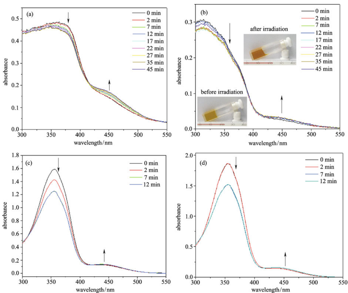
Figure 3 Absorption spectra of the thin films of (a) 1a and (b) Zn-1a ( 16.5\ \mu\text{m} ); and the solution of (c) 1b and (d) Zn-1b ( c = 1 \times 10^{-3}\ \text{mg}\cdot\text{mL}^{-1} , l = 0.1\ \text{cm} ) in DMSO upon 365 nm irradiation.
