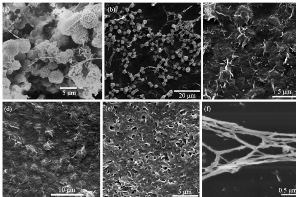
Figure 4 SEM images of Zn( m )- 1a : (a) m = 0 equiv, (b) m = 0.2 equiv, (c) m = 0.4 equiv, (d) m = 0.6 equiv, (e) m = 0.8 equiv and (f) m = 1.0 equiv from DMSO (40 mg · mL -1 ).
